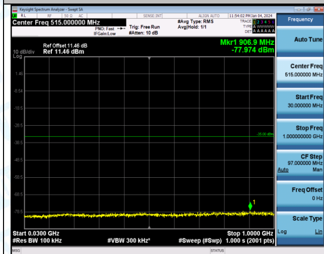
Band7_20MHz_16QAM_21350_1RB#0_20000~27000_20000~27000
