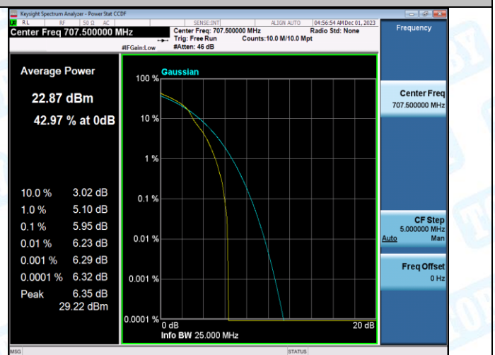
Band12-10MHz-16QAM-23095-50RB#0-PASS
