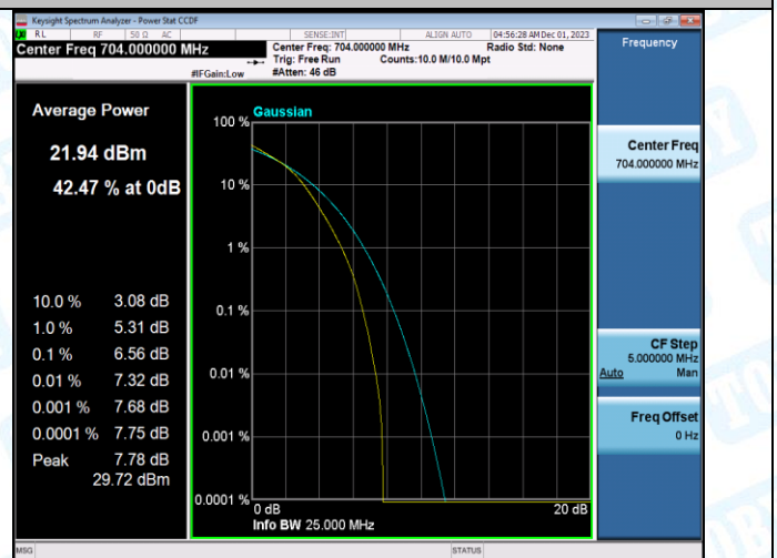
Band12-10MHz-16QAM-23095-1RB#0-PASS
