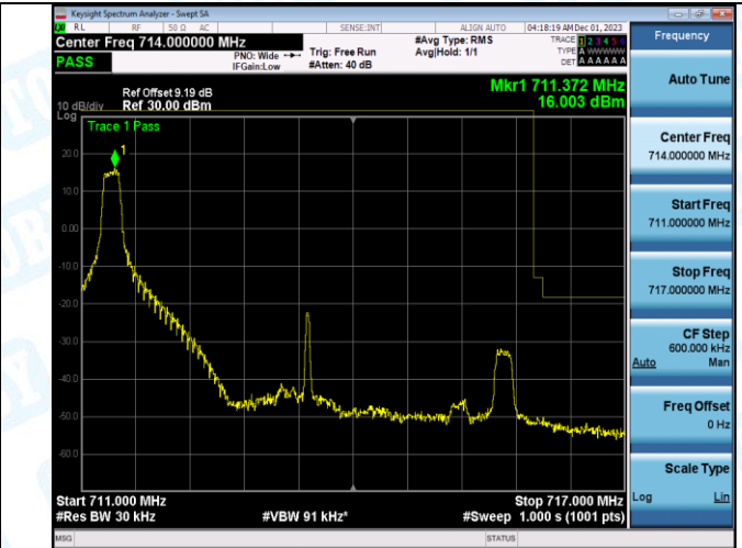
Band12_5MHz_16QAM_23155_1RB#24
