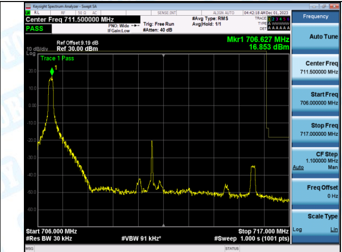
Band12_10MHz_16QAM_23130_1RB#49
