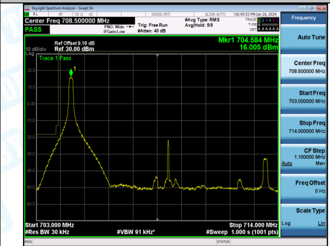
Band17_10MHz_16QAM_23780_50RB#0
