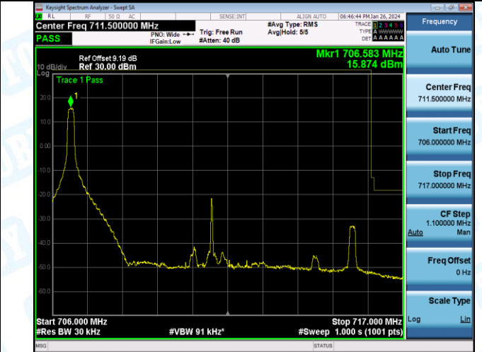
Band17_10MHz_16QAM_23800_50RB#0
