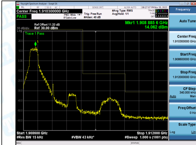
Band2_1.4MHz_QPSK_19193_1RB#5
