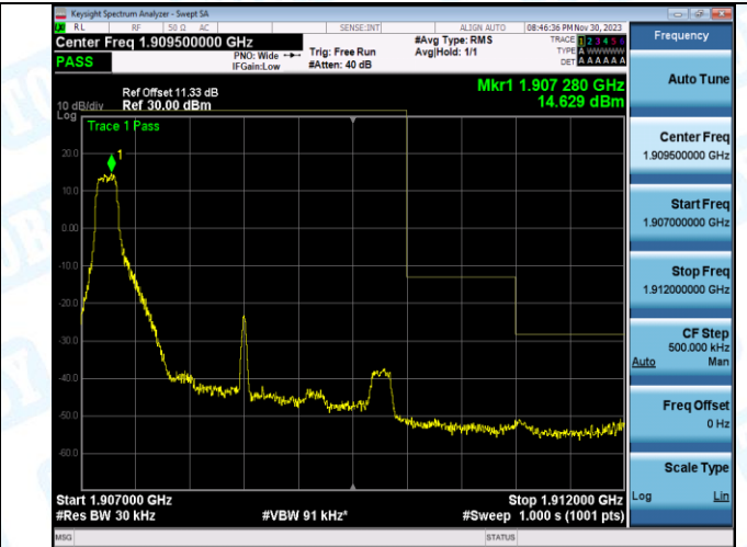
Band2_3MHz_16QAM_19185_1RB#14
