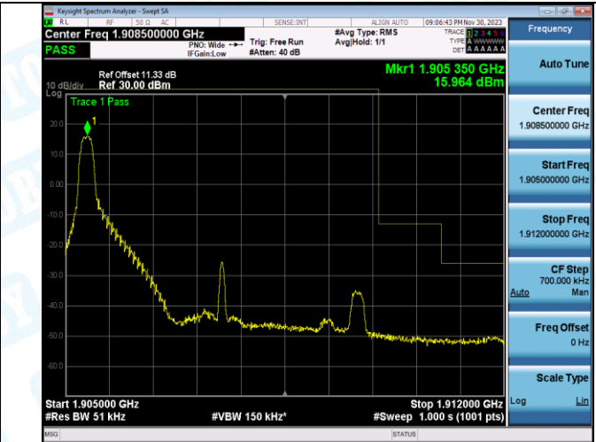
Band2_5MHz_16QAM_19175_1RB#24
