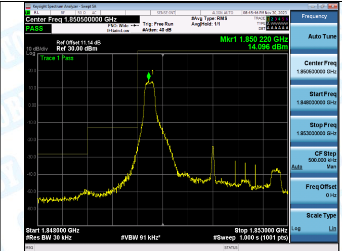
Band2_3MHz_16QAM_18615_1RB#14
