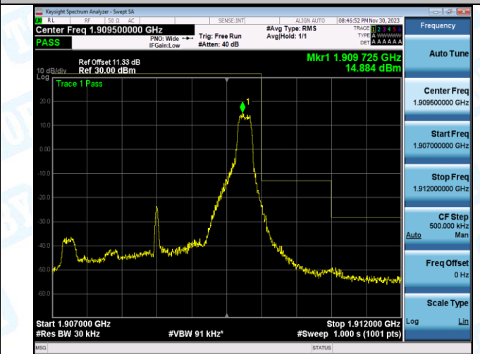
Band2_3MHz_16QAM_19185_15RB#0
