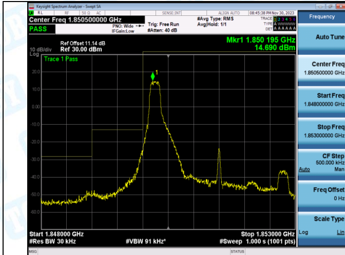
Band2_3MHz_QPSK_18615_1RB#14
