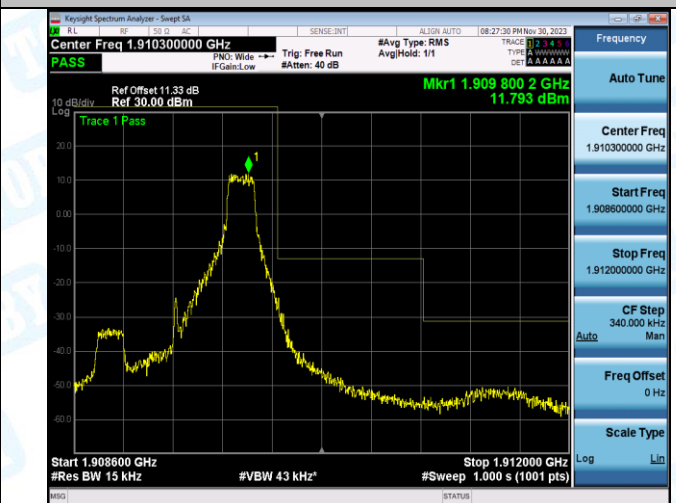
Band2_1.4MHz_16QAM_19193_6RB#0
