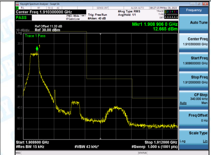
Band2_1.4MHz_16QAM_19193_1RB#5
