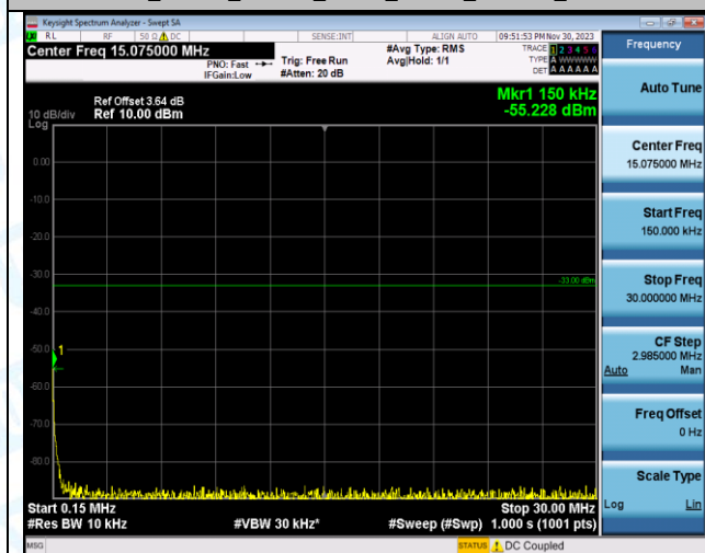
Band2_15MHz_16QAM_19125_1RB#0_1000~3000_1000~3000
