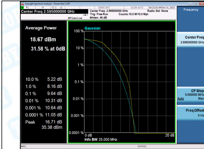
Band38-15MHz-QPSK-38175-1RB#0-PASS
