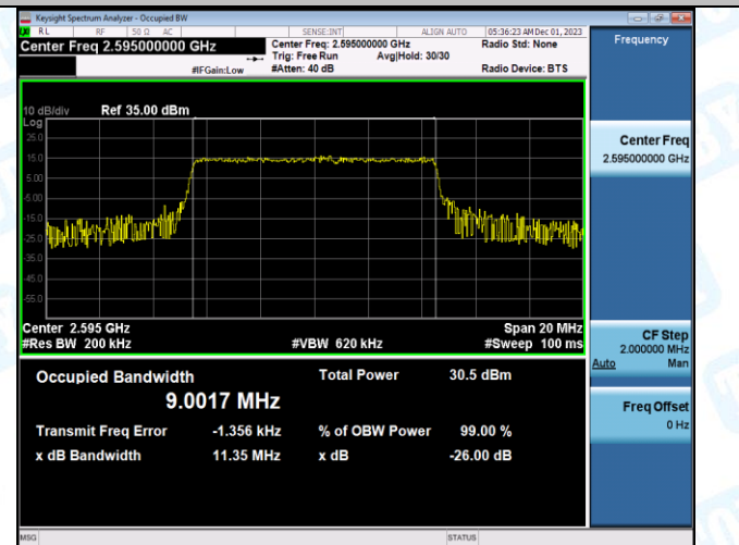
Band38-10MHz-16QAM-38200-50RB#0-PASS
