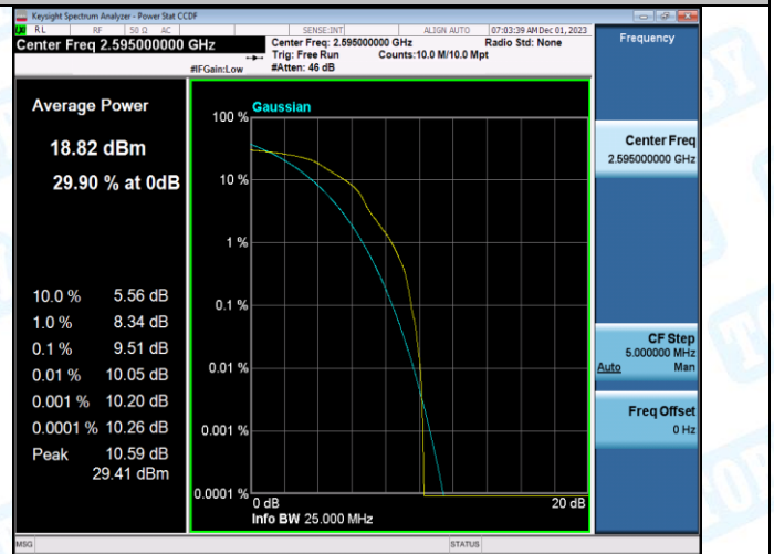
Band38-20MHz-16QAM-38000-100RB#0-PASS
