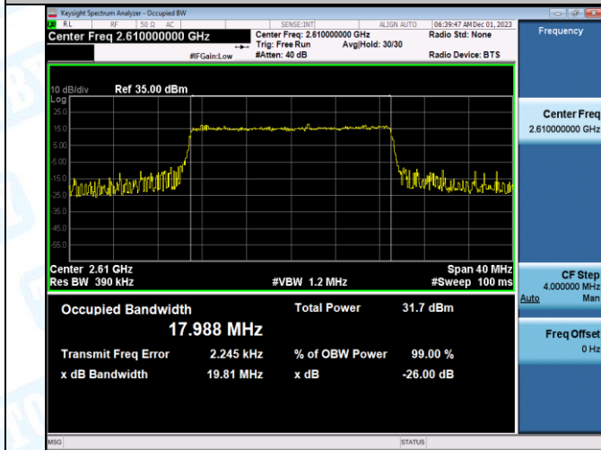
Band38-20MHz-QPSK-38150-100RB#0-PASS
