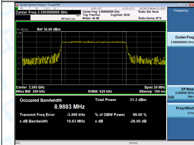
Band38-10MHz-QPSK-38200-50RB#0-PASS
