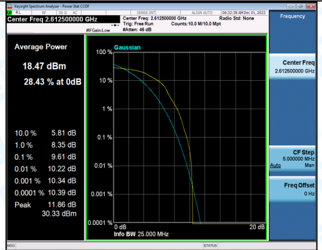
Band38-15MHz-16QAM-38175-75RB#0-PASS
