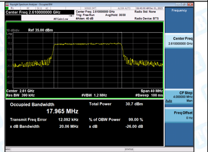
Band38-20MHz-16QAM-38150-100RB#0-PASS
