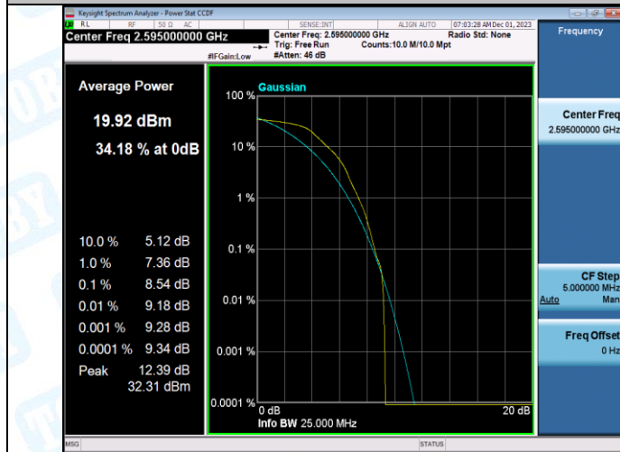
Band38-20MHz-QPSK-38000-100RB#0-PASS
