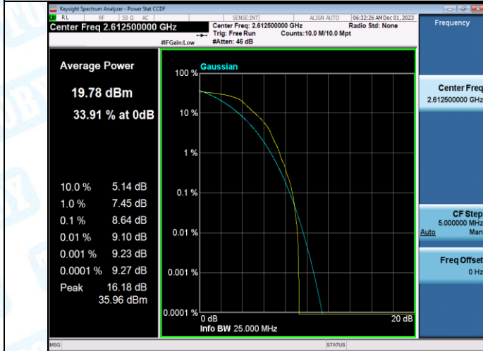
Band38-15MHz-QPSK-38175-75RB#0-PASS
