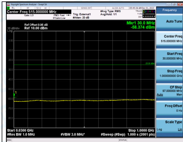
Band38_10MHz_QPSK_38000_1RB#0_20000~27000_20000~27000
