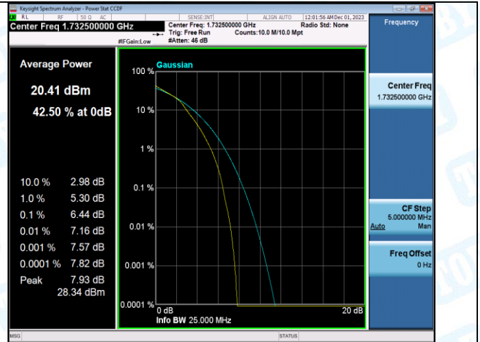
Band4-15MHz-16QAM-20325-1RB#0-PASS
