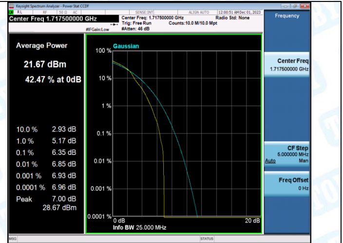
Band4-15MHz-16QAM-20025-75RB#0-PASS
