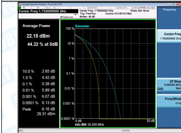
Band4-10MHz-QPSK-20350-50RB#0-PASS
