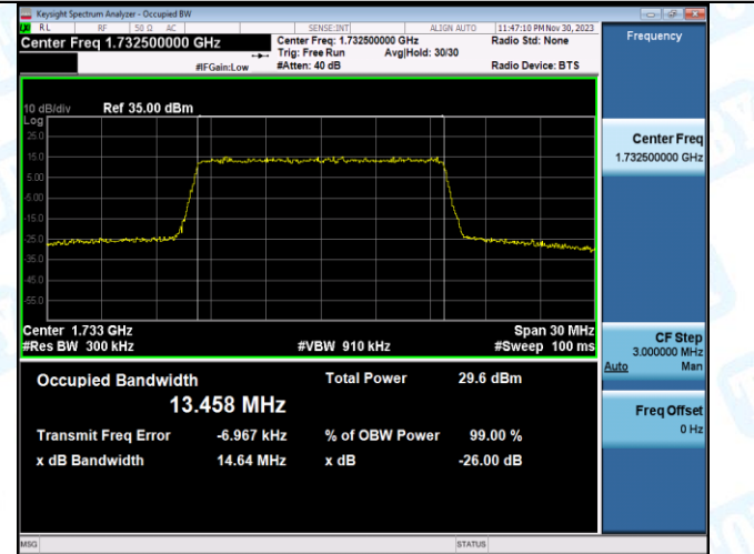
Band4-15MHz-16QAM-20325-75RB#0-PASS
