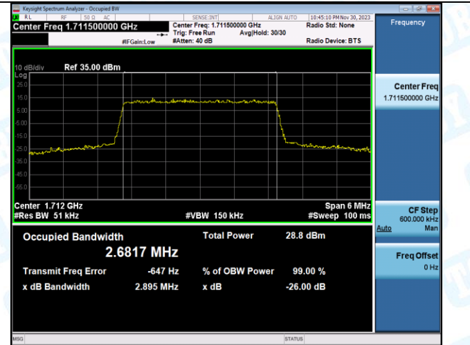
Band4-3MHz-16QAM-20175-15RB#0-PASS
