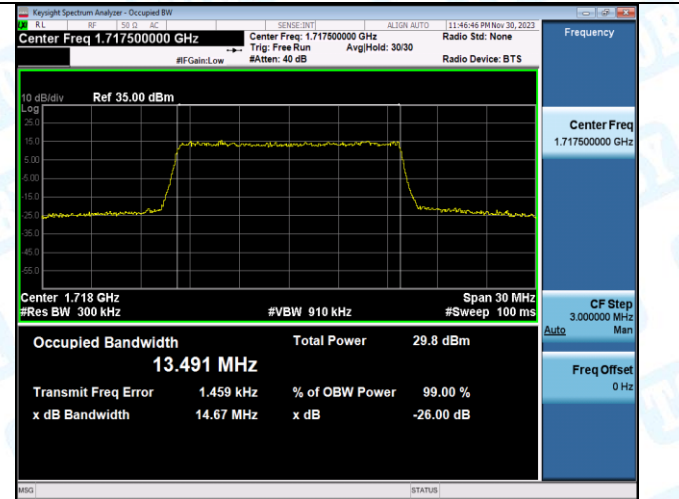
Band4-15MHz-16QAM-20175-75RB#0-PASS
