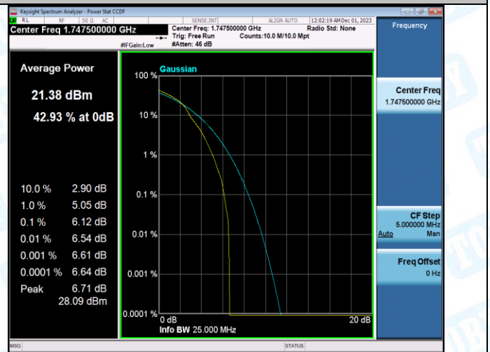
Band4-15MHz-16QAM-20325-75RB#0-PASS
