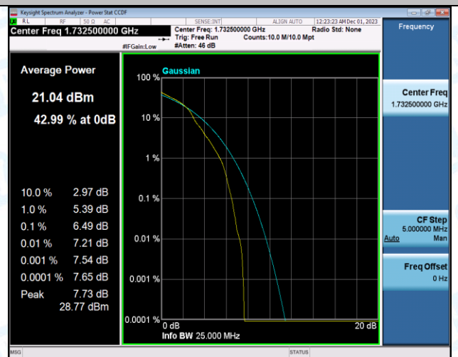
Band4-20MHz-16QAM-20175-100RB#0-PASS
