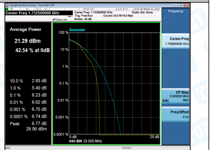
Band4-15MHz-16QAM-20175-75RB#0-PASS
