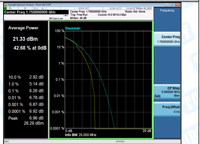
Band4-10MHz-16QAM-20350-50RB#0-PASS
