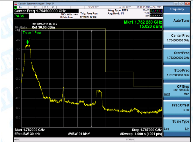
Band4_3MHz_16QAM_20385_1RB#14
