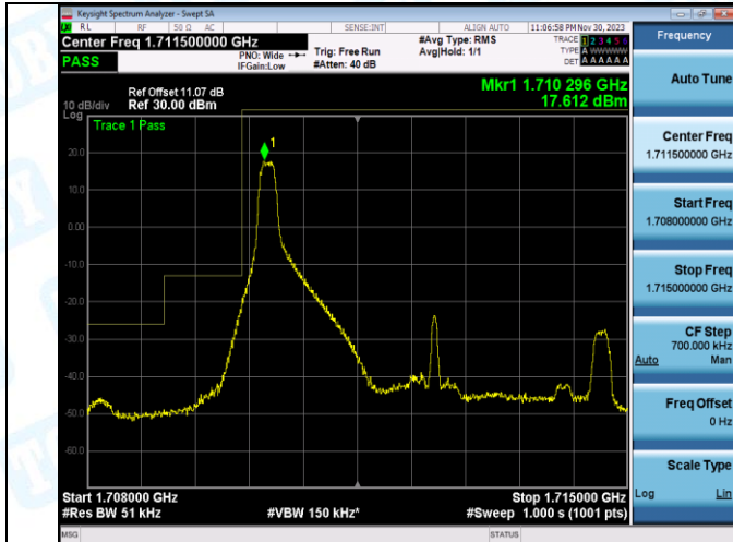
Band4_5MHz_QPSK_19975_1RB#24
