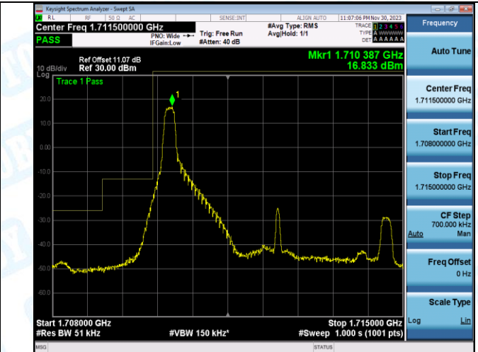
Band4_5MHz_16QAM_19975_1RB#24
