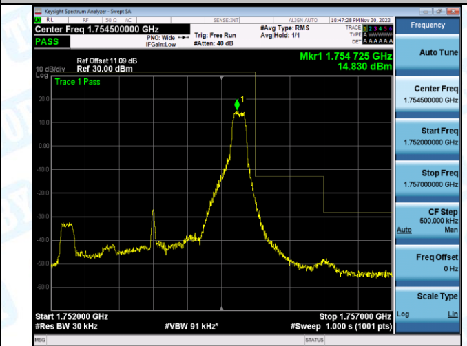
Band4_3MHz_16QAM_20385_15RB#0
