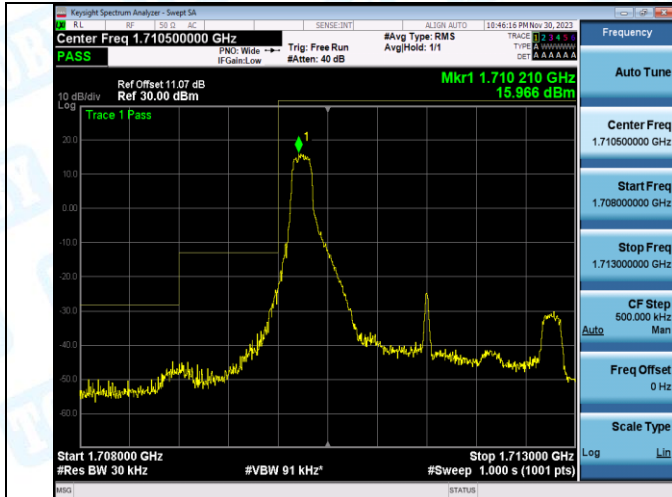
Band4_3MHz_QPSK_19965_1RB#14
