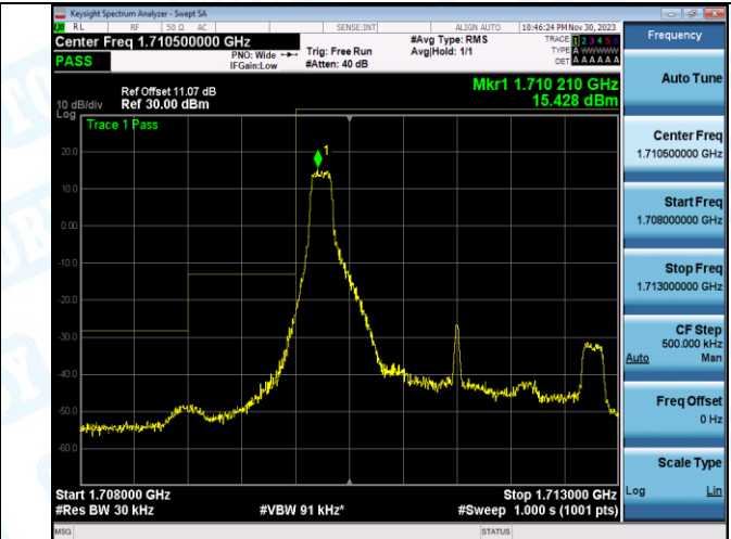
Band4_3MHz_16QAM_19965_1RB#14
