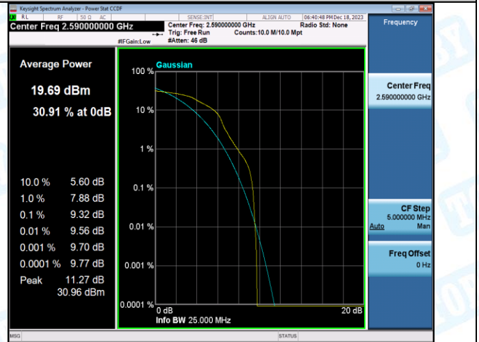
41(2535-2655)-15MHz-16QAM-40590-75RB#0-PASS
