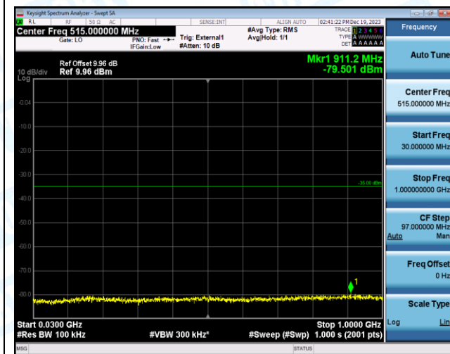
Band41_5MHz_QPSK_40065_1RB#0_20000~27000_20000~27000
