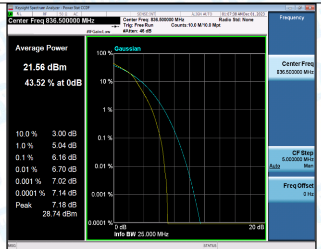
Band5-3MHz-16QAM-20635-1RB#0-PASS
