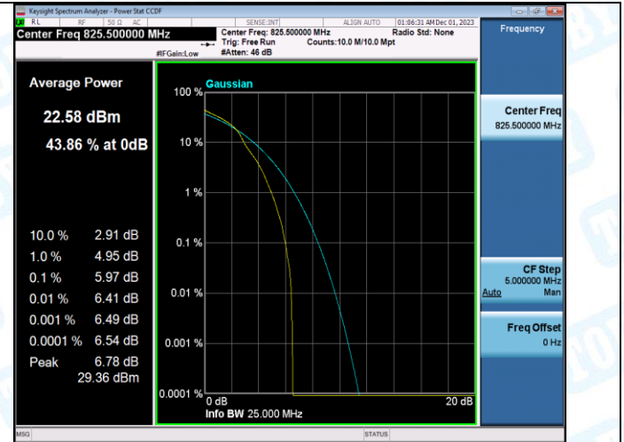
Band5-3MHz-16QAM-20415-15RB#0-PASS
