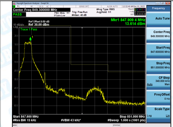
Band5_1.4MHz_16QAM_20643_1RB#5
