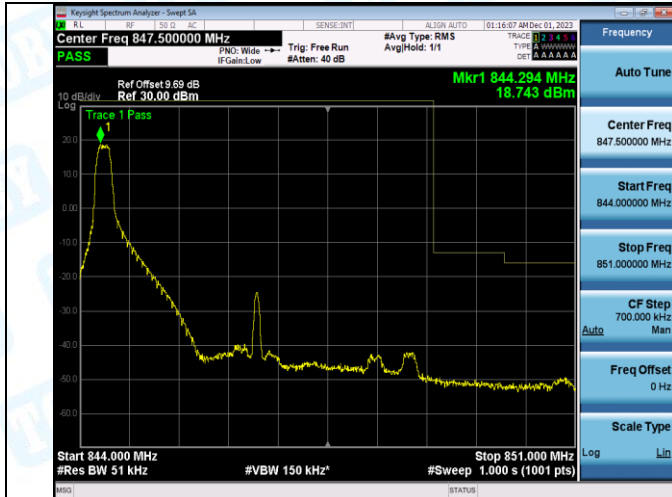
Band5_5MHz_QPSK_20625_1RB#24
