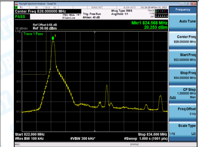
Band5_10MHz_16QAM_20450_1RB#49
