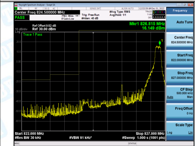
Band5_3MHz_16QAM_20415_15RB#0
