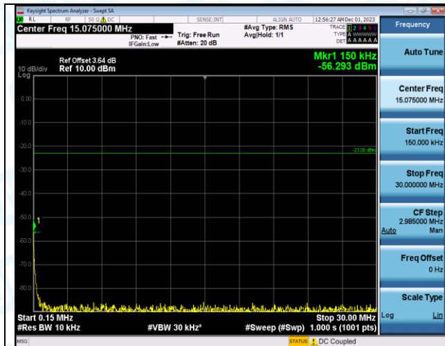
Band5_3MHz_16QAM_20415_1RB#0_1000~3000_1000~3000
