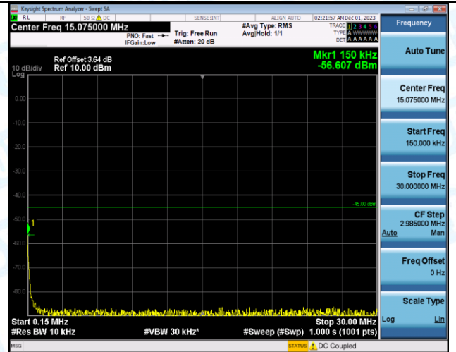
Band7_10MHz_QPSK_20800_1RB#0_1000~20000_1000~20000
