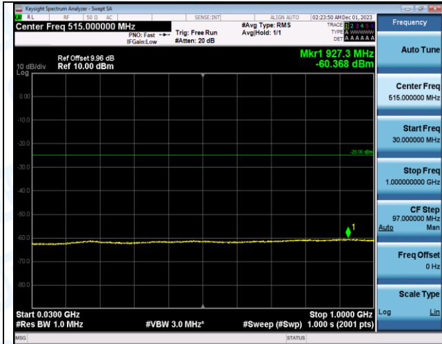
Band7_10MHz_QPSK_21100_1RB#0_20000~27000_20000~27000
