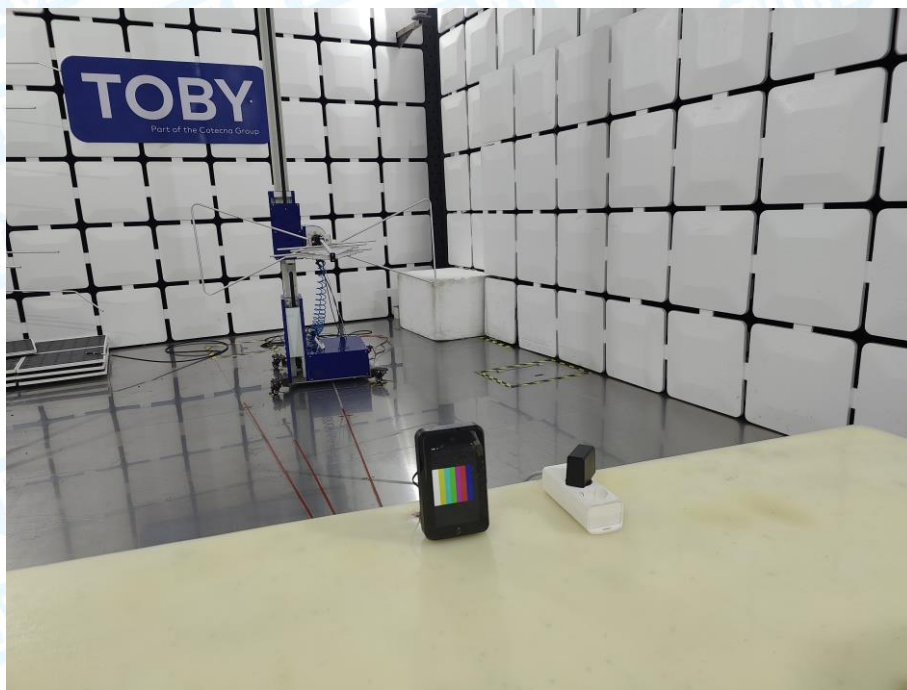
Photo of Setup for Radiated Emission (Above 1 GHz) ----Internal
