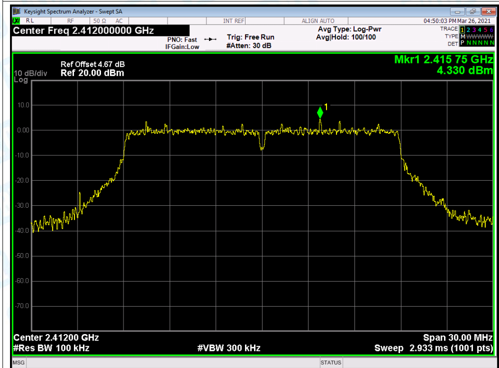
Band Edge NVNT n(HT20) 2412MHz Ant1 Emission
