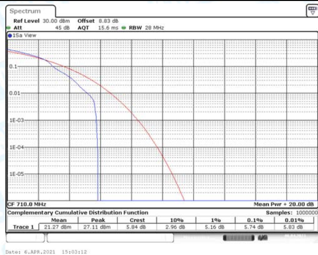
Band17-5MHz-16QAM-23790-25RB#0
