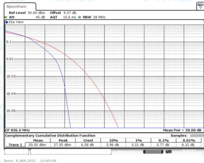
Band5-5MHz-16QAM-20625-25RB#0
