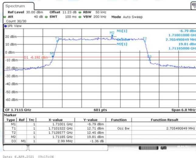
Band4-3MHz-QPSK-20175-15RB#0
