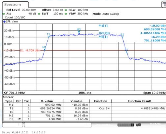
Band12-5MHz-16QAM-23095-25RB#0
