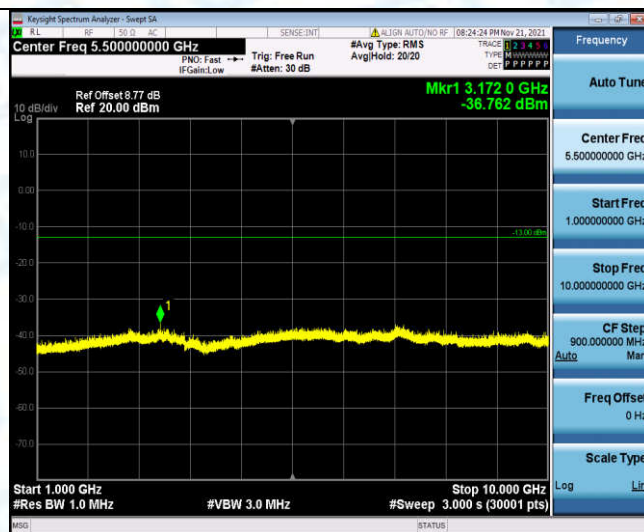
Band5-4183-3-1000~10000MHz
