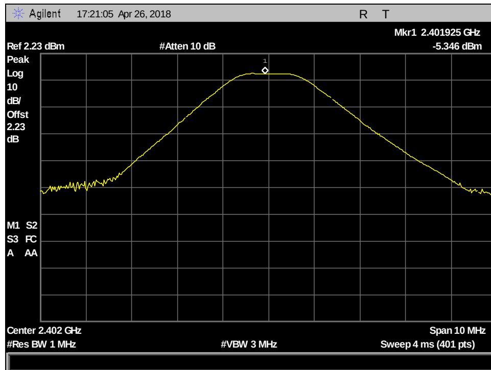
Plot 4. Peak Power Output, Low Channel
