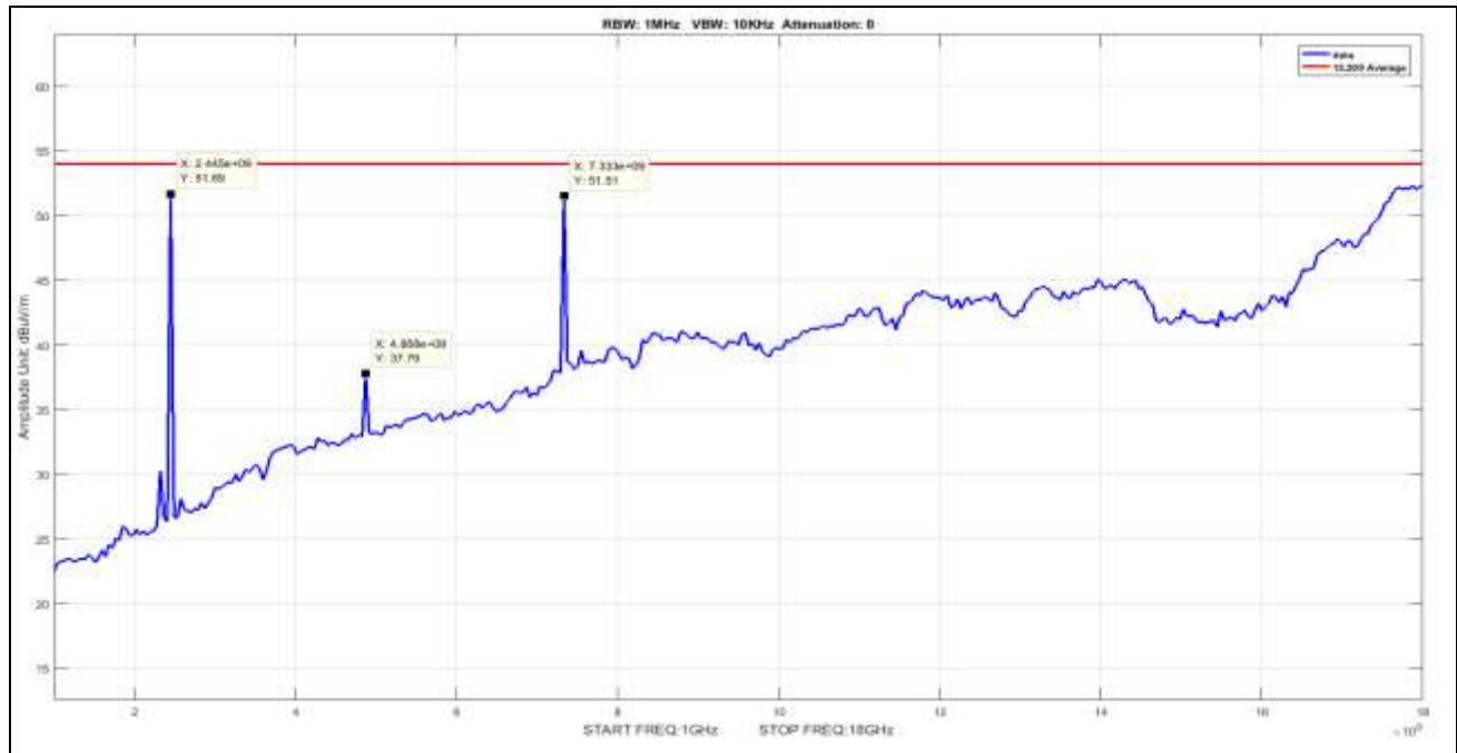
Plot 10. Radiated Spurious Emissions, Mid Channel, 1 – 18 GHz, Average
