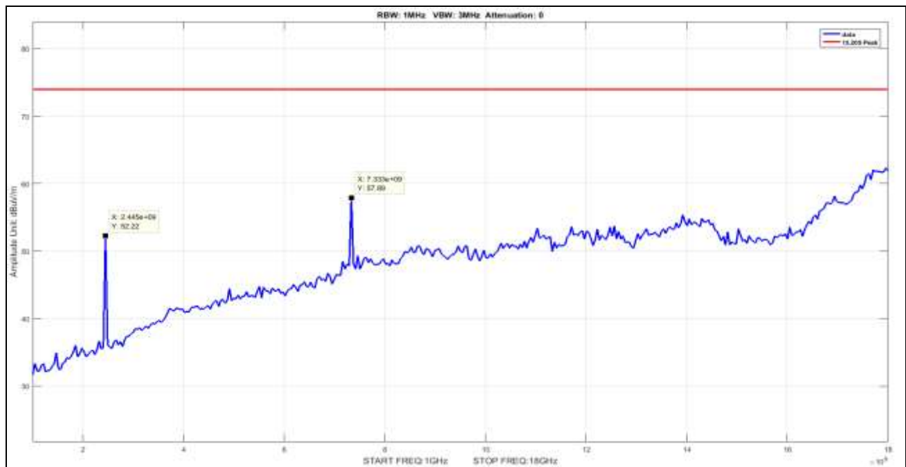
Plot 11. Radiated Spurious Emissions, Mid Channel, 1 GHz – 18 GHz, Peak
