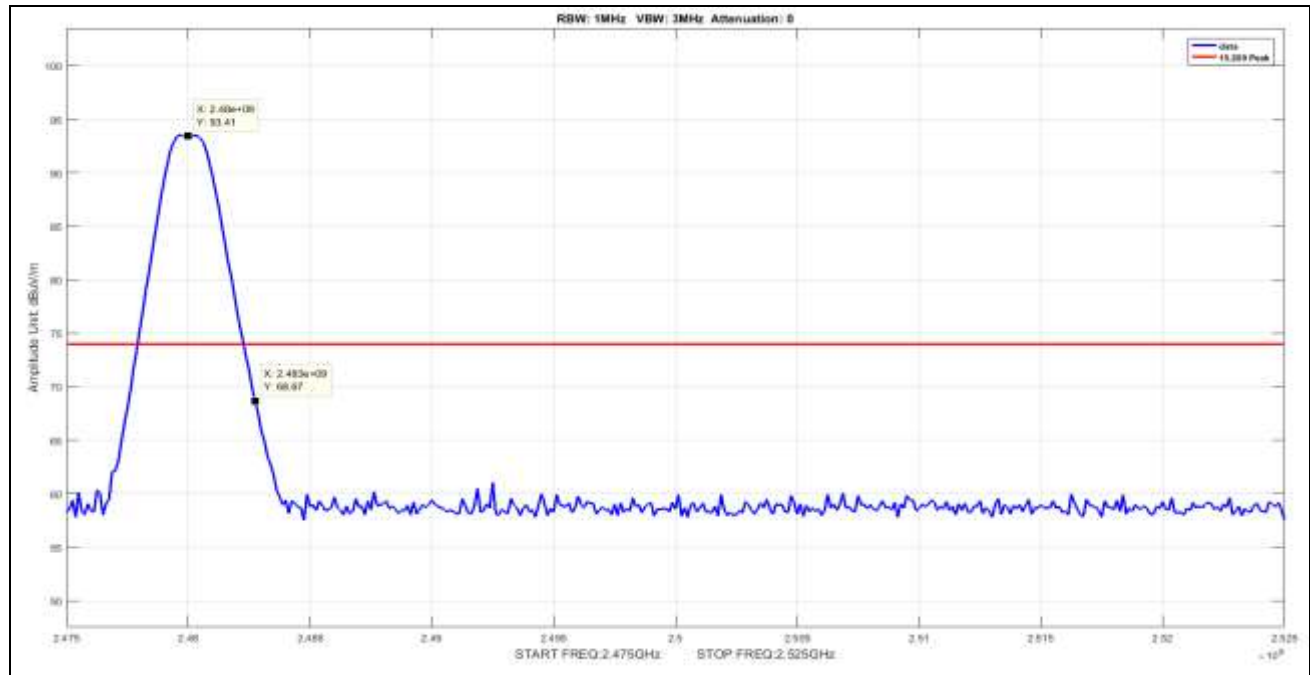
Plot 17. Radiated Restricted Band Edge, High Channel, Peak
