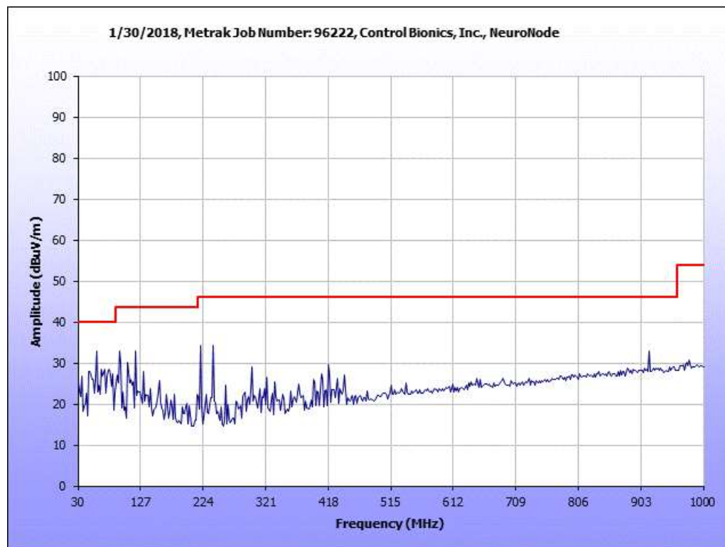
Plot 7. Radiated Spurious Emissions 30 MHz - 1 GHz, Prescan
