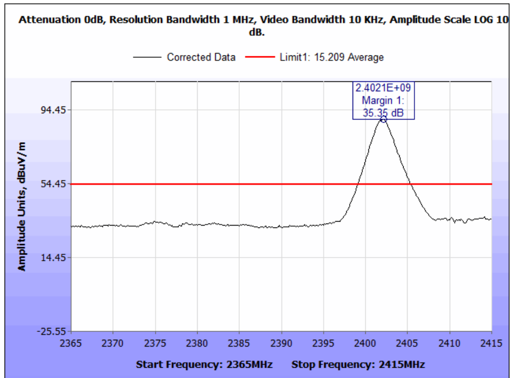
Plot 14. Radiated Restricted Band Edge, Low Channel, Average
