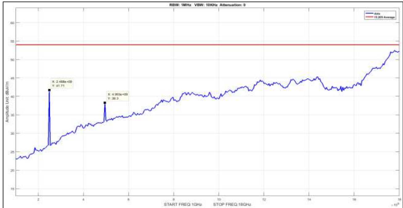
Plot 12. Radiated Spurious Emissions, High Channel, 1 – 18 GHz, Average
