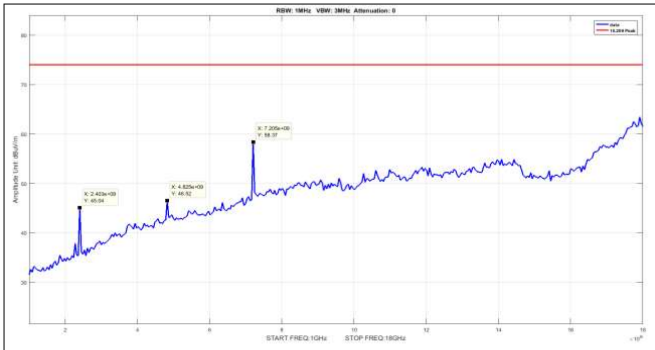
Plot 9. Radiated Spurious Emissions, Low Channel, 1 GHz – 18 GHz, Peak
