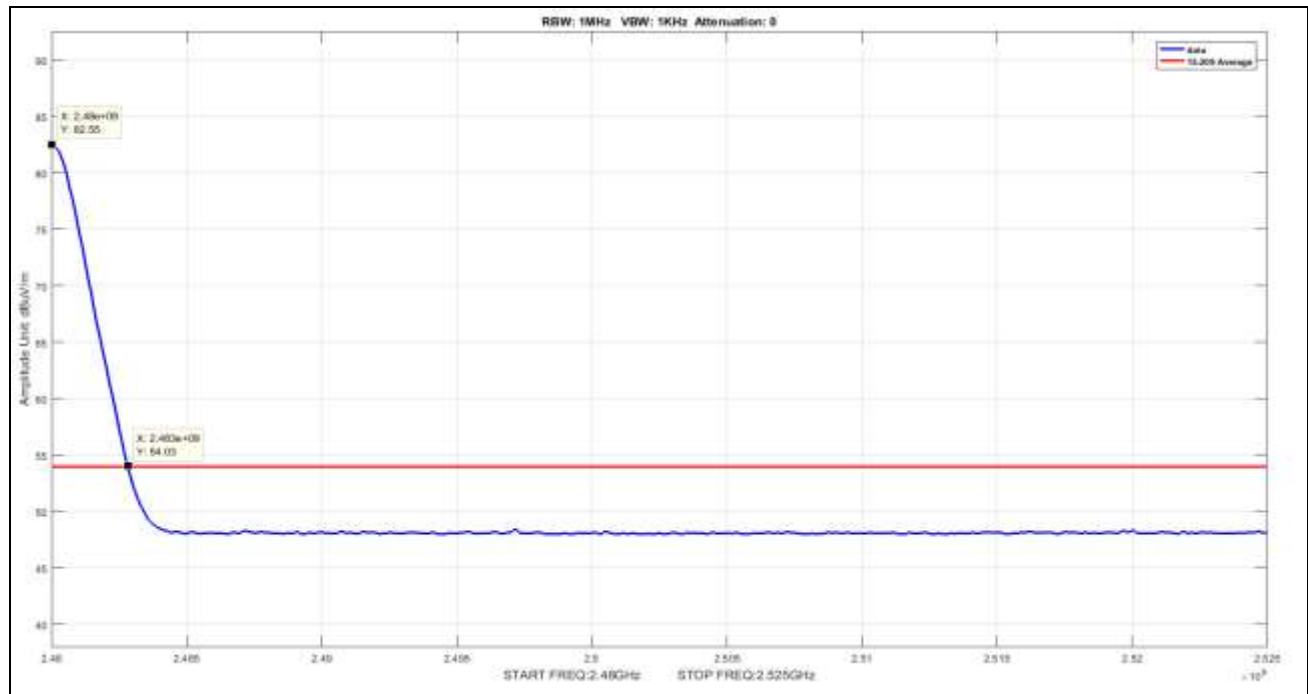
Plot 16. Radiated Restricted Band Edge, High Channel, Average
