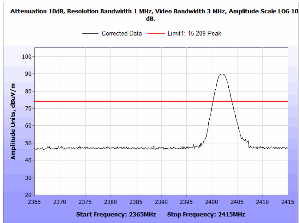
Plot 15. Radiated Restricted Band Edge, Low Channel, Peak
