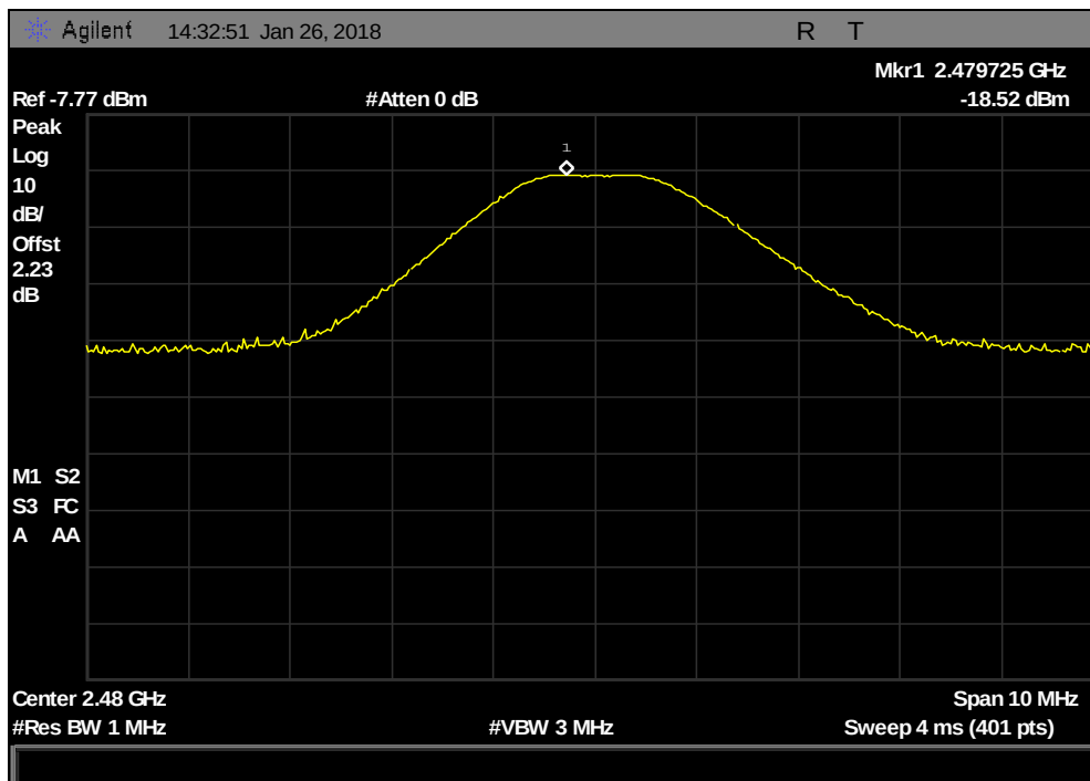
Plot 6. Peak Power Output, High Channel
