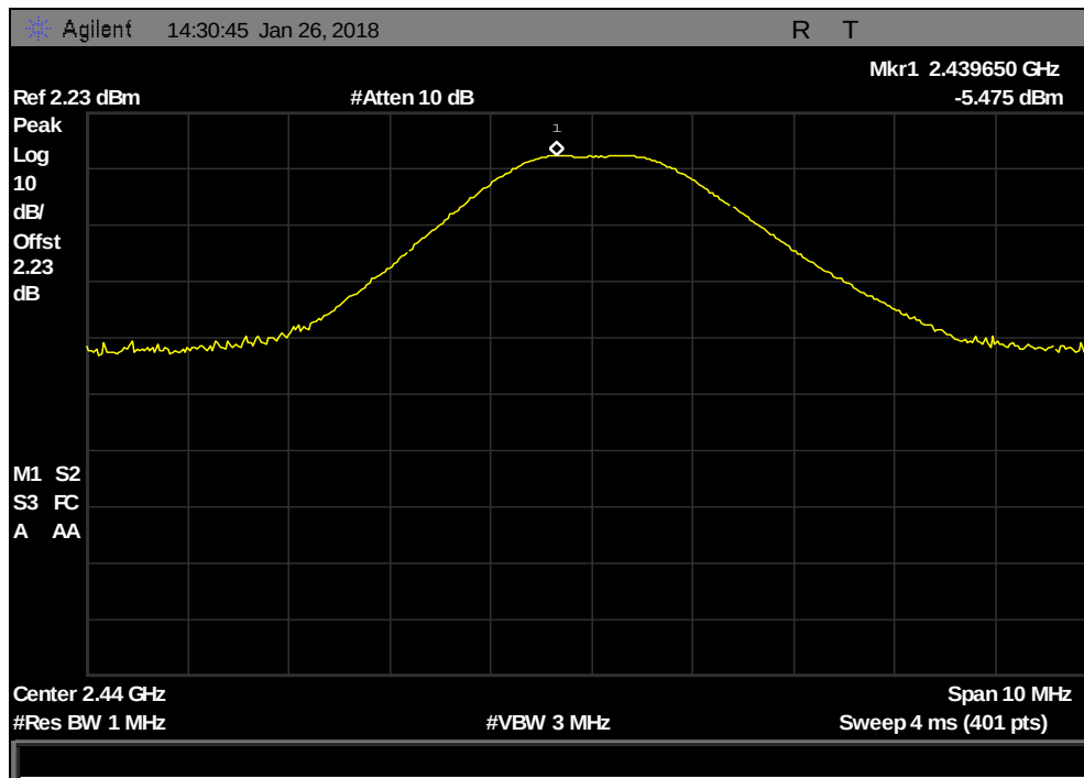
Plot 5. Peak Power Output, Mid Channel
