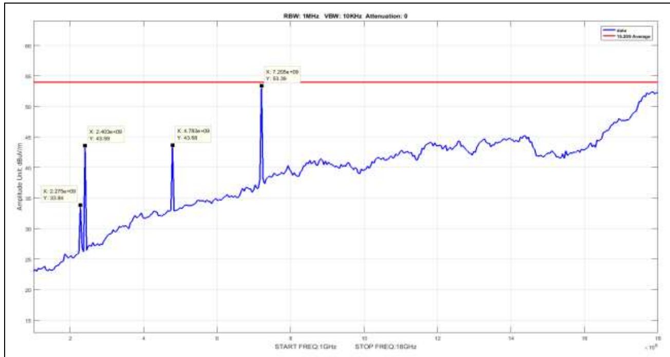
Plot 8. Radiated Spurious Emissions, Low Channel, 1 – 18 GHz, Average
