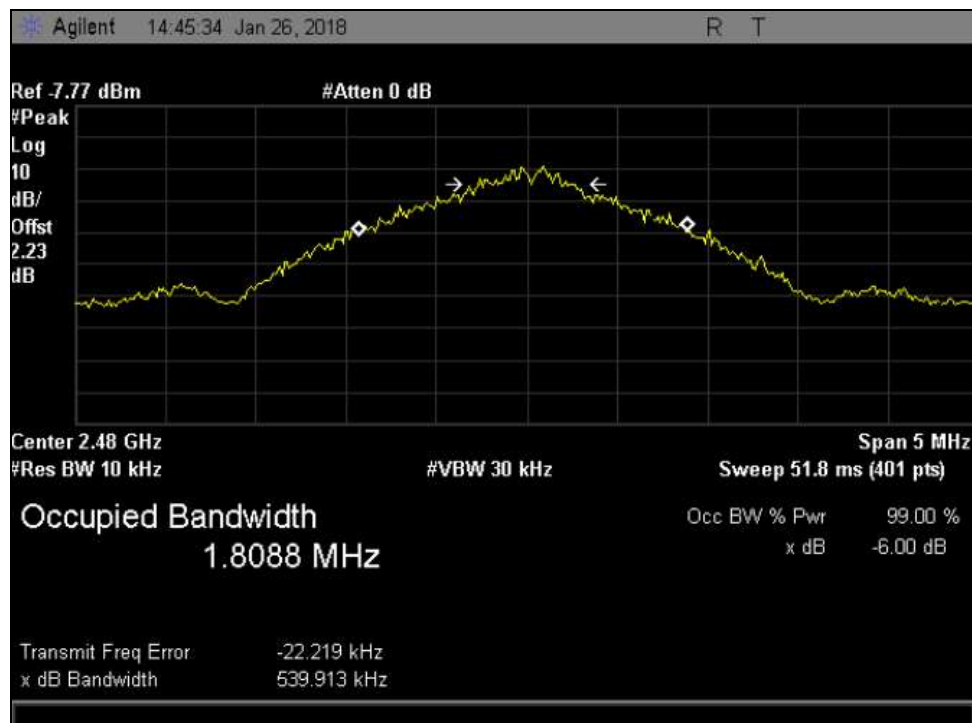
Plot 3. 99% Occupied Bandwidth, High Channel
