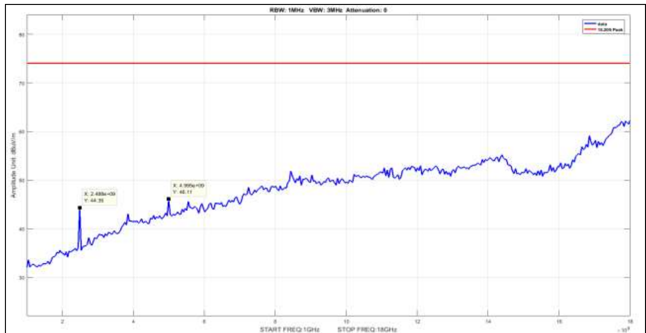
Plot 13. Radiated Spurious Emissions, High Channel, 1 GHz – 18 GHz, Peak
