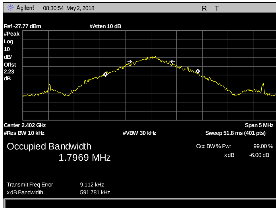
Plot 1. 99% Occupied Bandwidth, Low Channel
