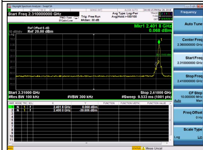
8DPSK-Left Side
