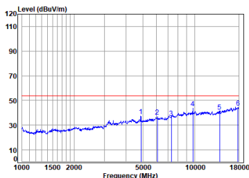
BLE_1M_TX_CH_19_Vertical-Avg
