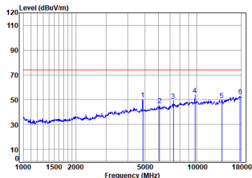
BLE_1M_TX_CH_19_Horizontal-Peak
