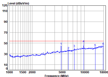
BLE_1M_TX_CH_19_Horizontal-Avg
