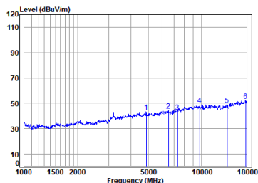
BLE_1M_TX_CH_19_Vertical-Peak
