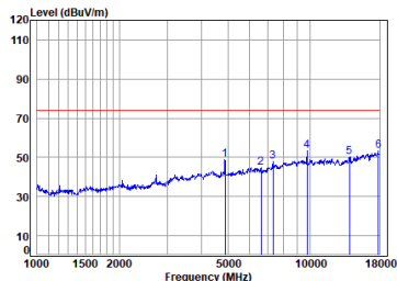
BLE_2M_TX_CH_19_Horizontal-Peak
