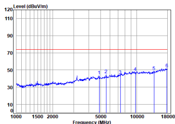
BLE_2M_TX_CH_19_Vertical-Peak
