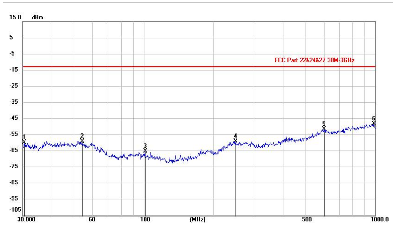
(LTE Band 41_QPSK_ Middle Channel _ 30MHz to 1GHz _Horizontal)
