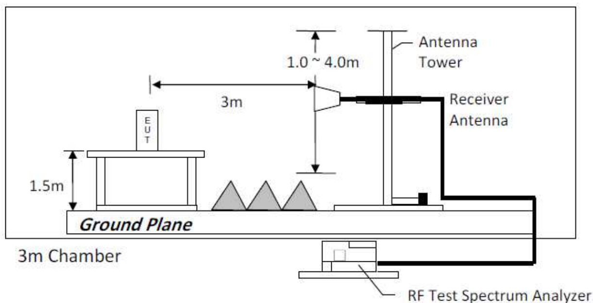
Test setup of radiated emissions above 1GHz
