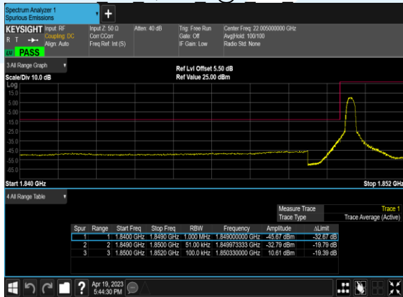
B25 5M 16QAM 1@0 CH 26065
