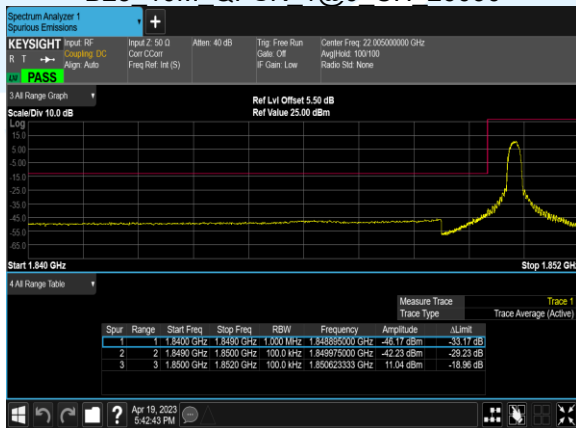
B25 10M 16QAM 1@0 CH 26090
