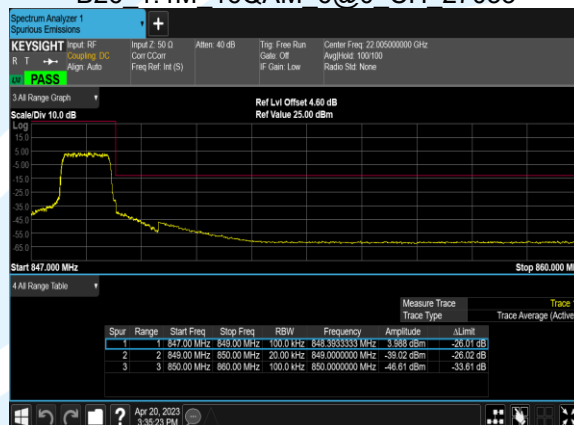
B26 1.4M 16QAM 6@0 CH 27033
