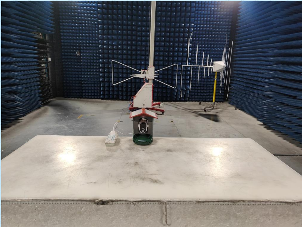
Radiated Emission Below 1GHz Test Setup
