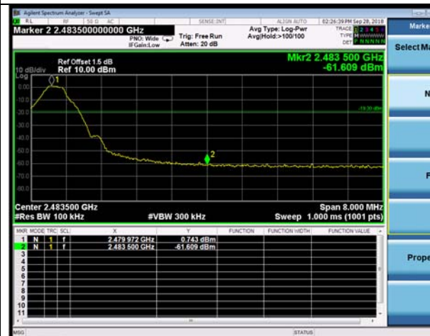
GFSK,2480MHz,DH5,Plot 1,Band Edge
