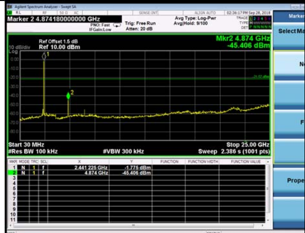
DQPSK,2441MHz,2DH5,Plot 2, 30MHz~25000MHz
