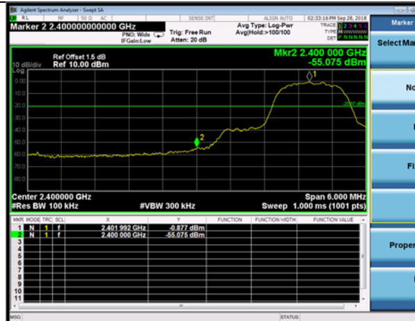
DQPSK,2402MHz,2DH5,Plot 1,Band Edge
