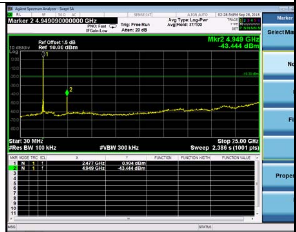
GFSK,2480MHz,DH5, Plot 2, 30MHz~25000MHz
