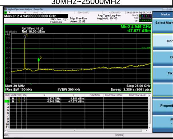
DQPSK,2480MHz,2DH5,Plot 2, 30MHz~25000MHz
