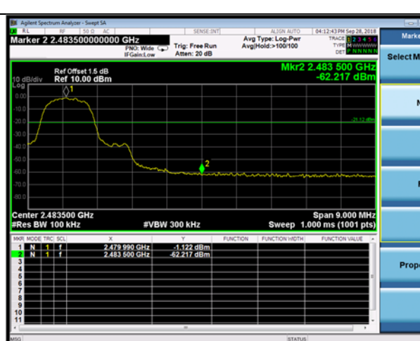
DQPSK,2480MHz,2DH5,Plot 1,Band Edge
