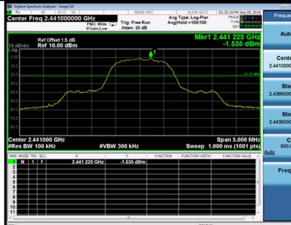
DQPSK,2441MHz,2DH5,Plot 1,Band Edge
