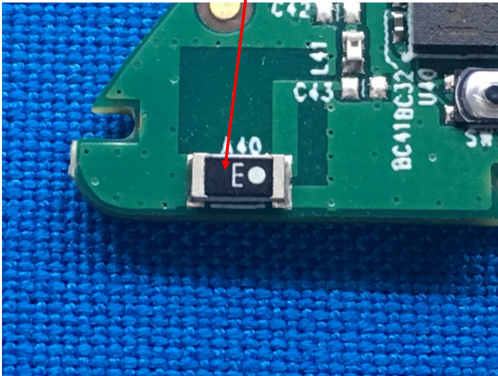
Chip Antenna – Top View
