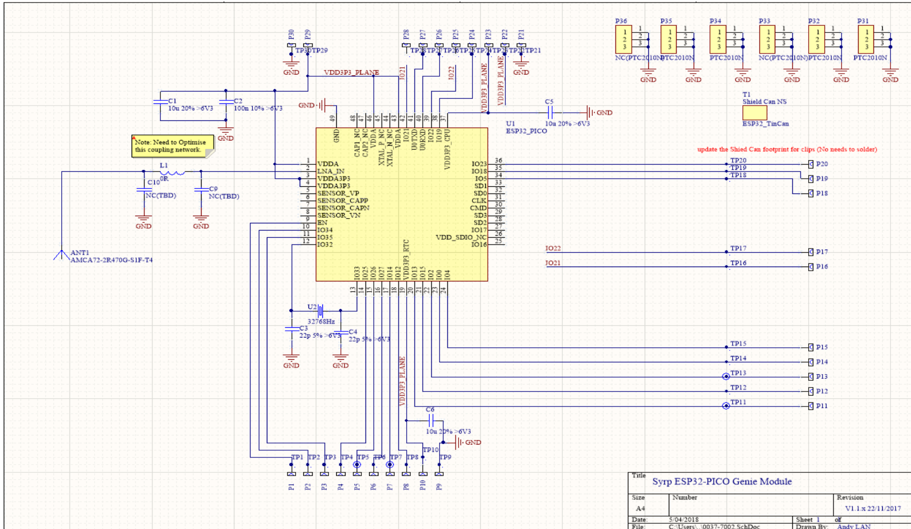
Figure 4: ESP32-0031-7002 Schematics
