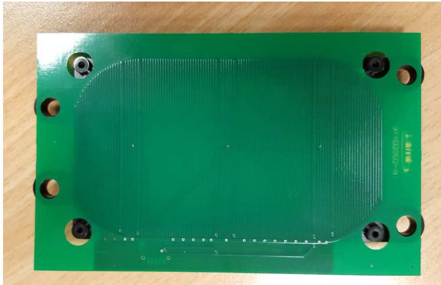
Coil Module
