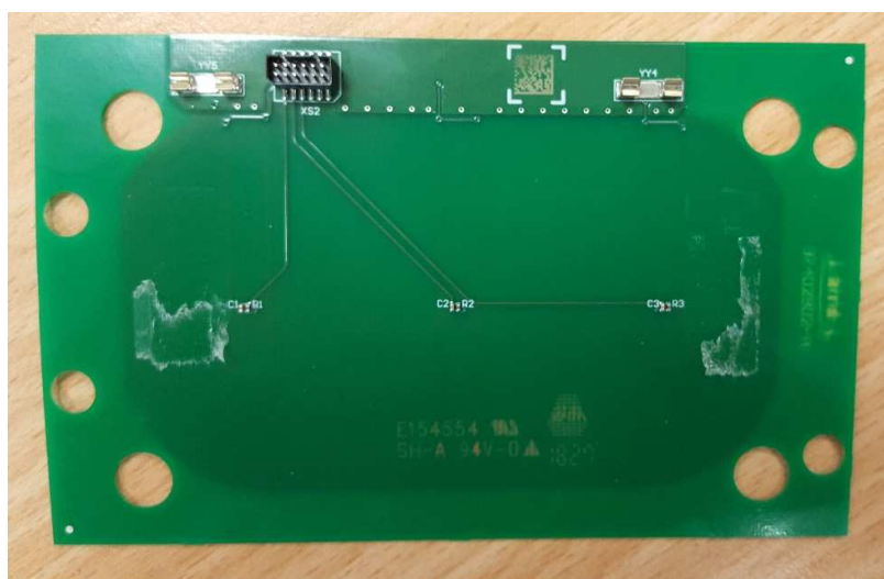
Cap Sensor Board top view
