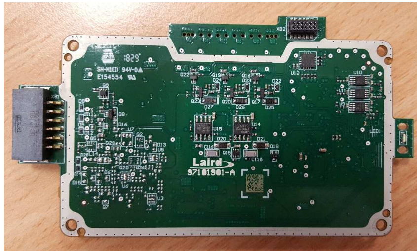
Main Board without shielding
