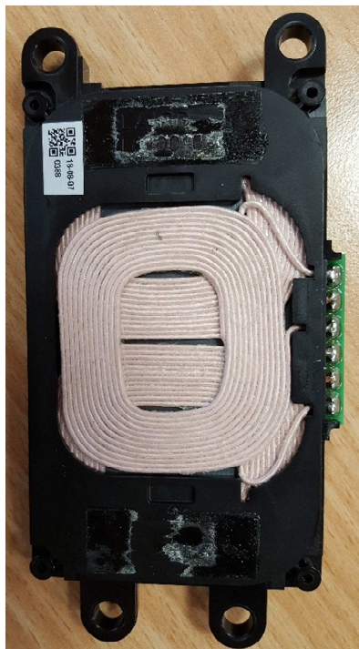
Coil Module
