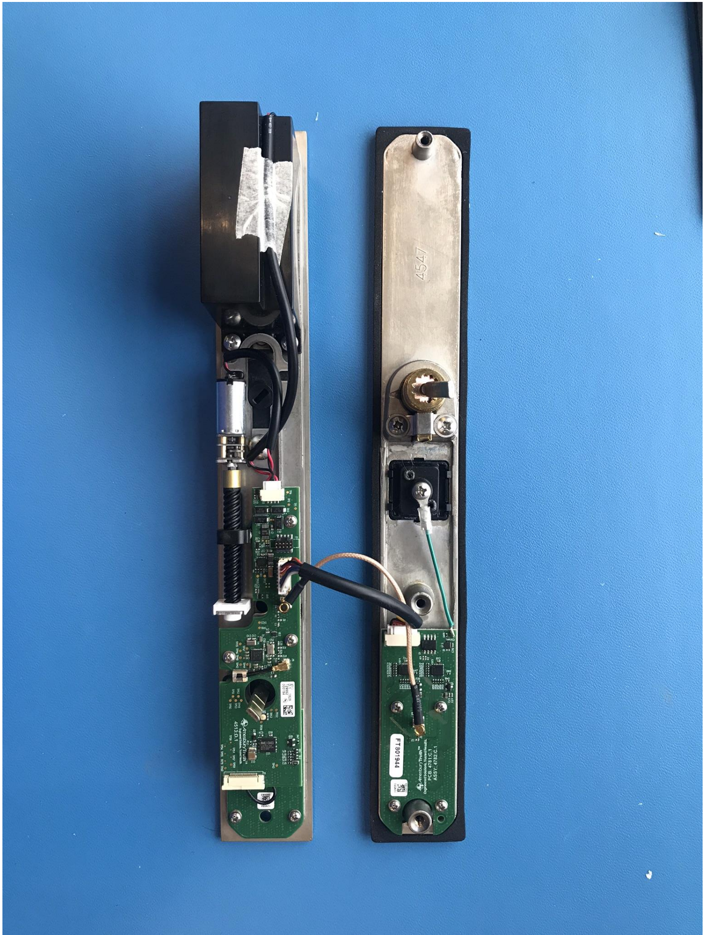
Figure 10 - Internal Assembly with Connections
