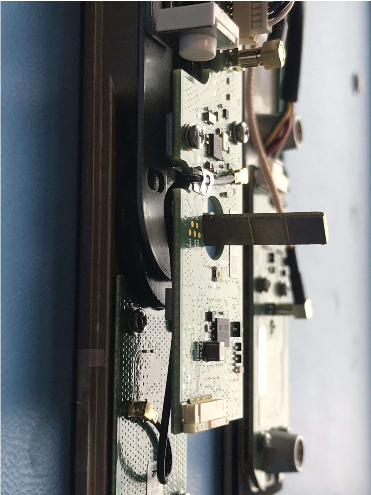
Figure 13 - Interior RF Connection
