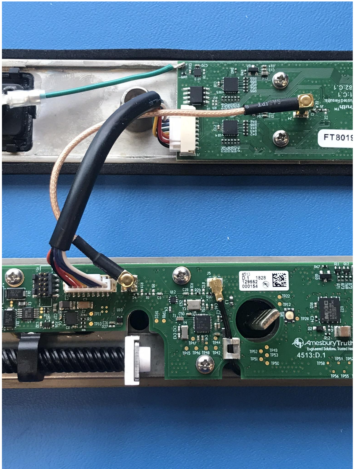
Figure 12 - Connections to Exterior Side, RF and Data
