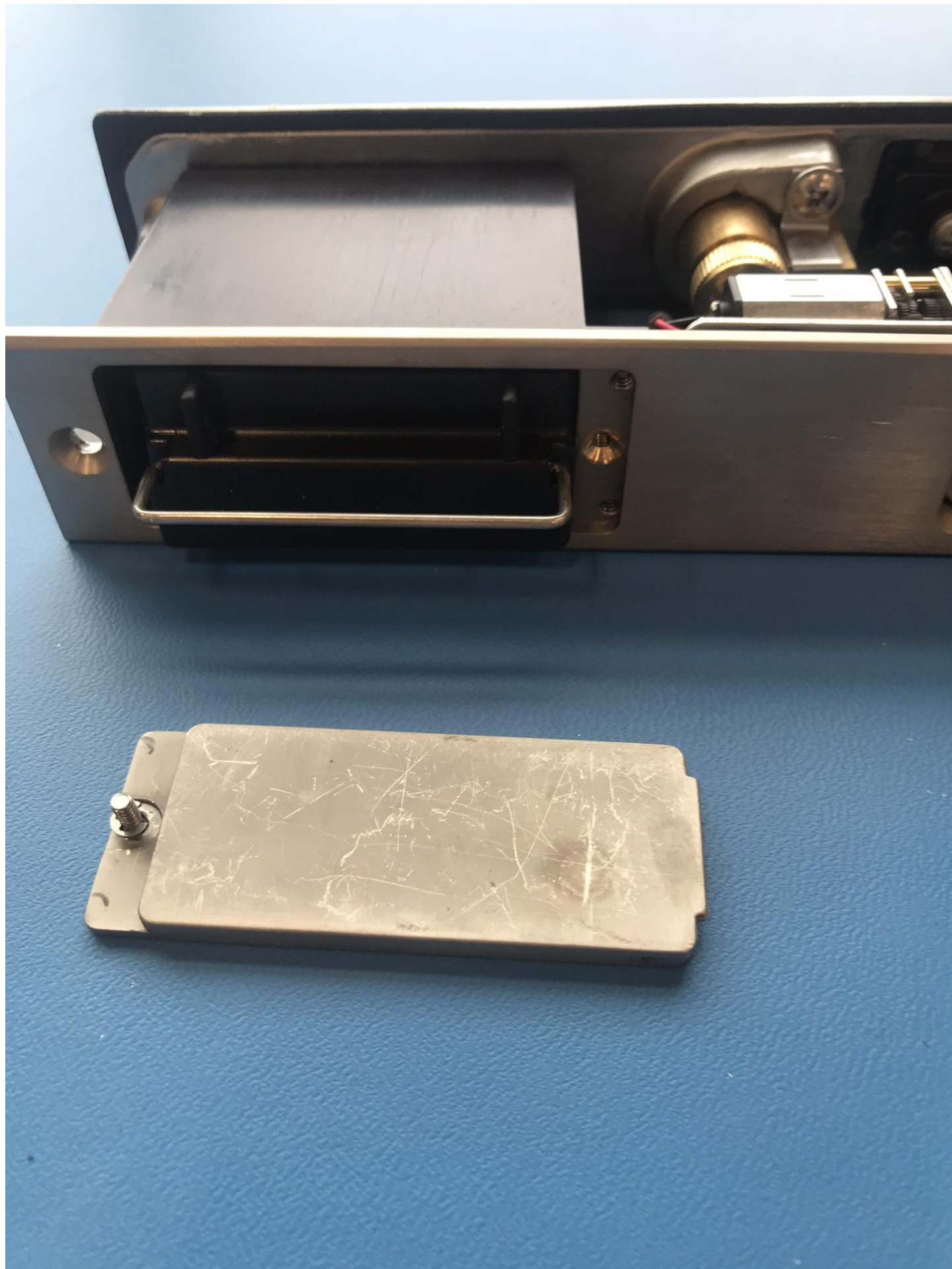
Figure 17 - Battery Compartment Open, Battery Cartridge Partially Removed
