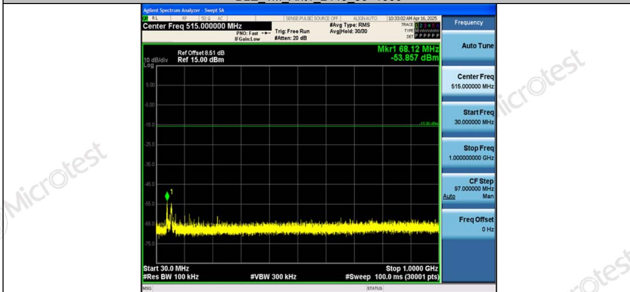
BLE_1M_Ant1_2440_30~1000
