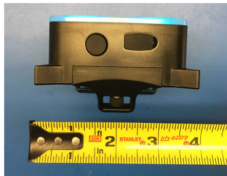
Fig 3: Front view.
