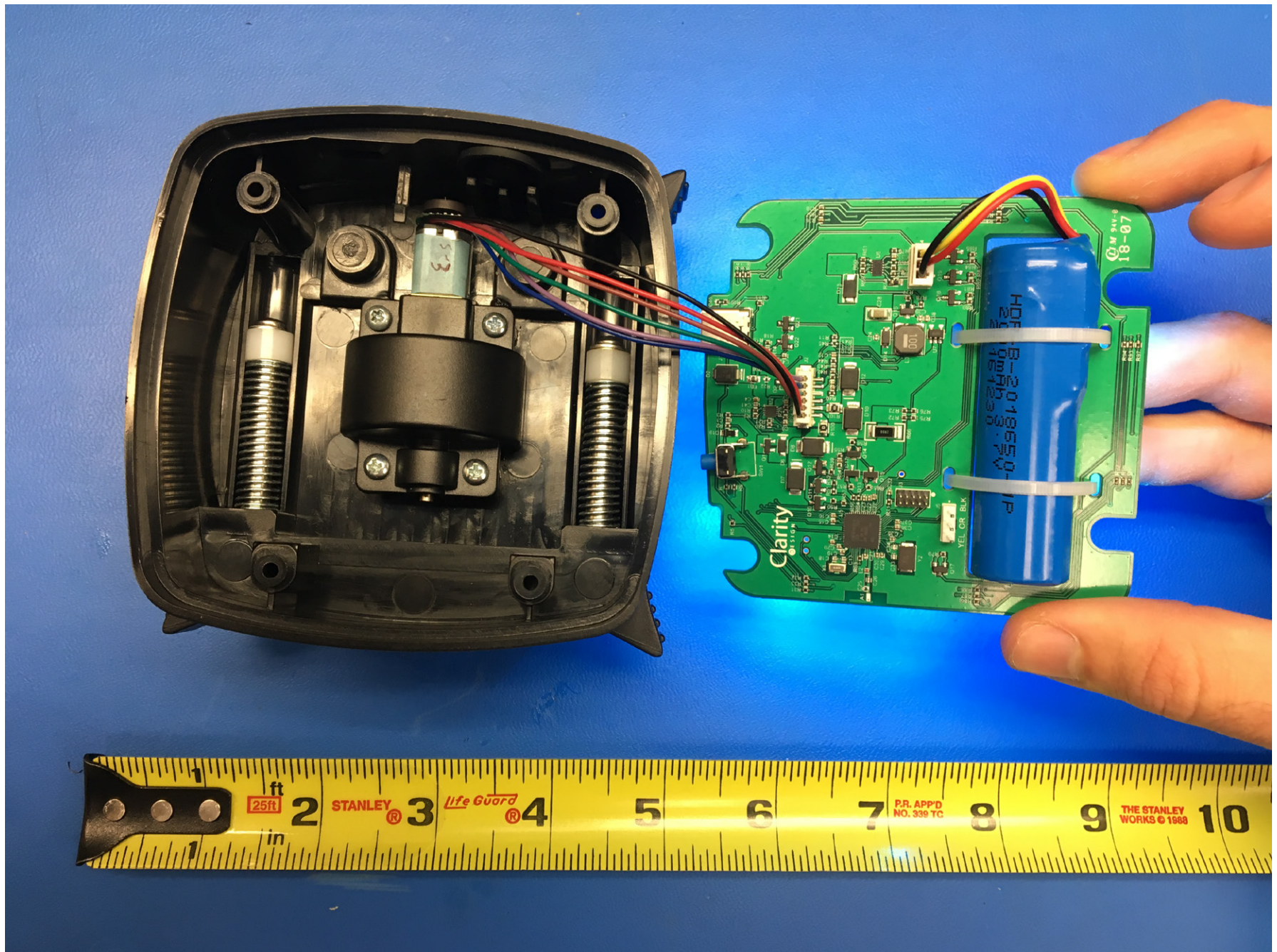
Fig 5: Top view of system with PCA connected but not assembled.
