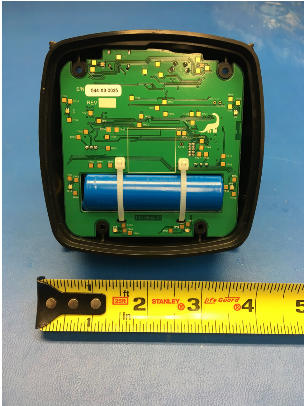
Fig 1: Top view of system with PCA assembled.
