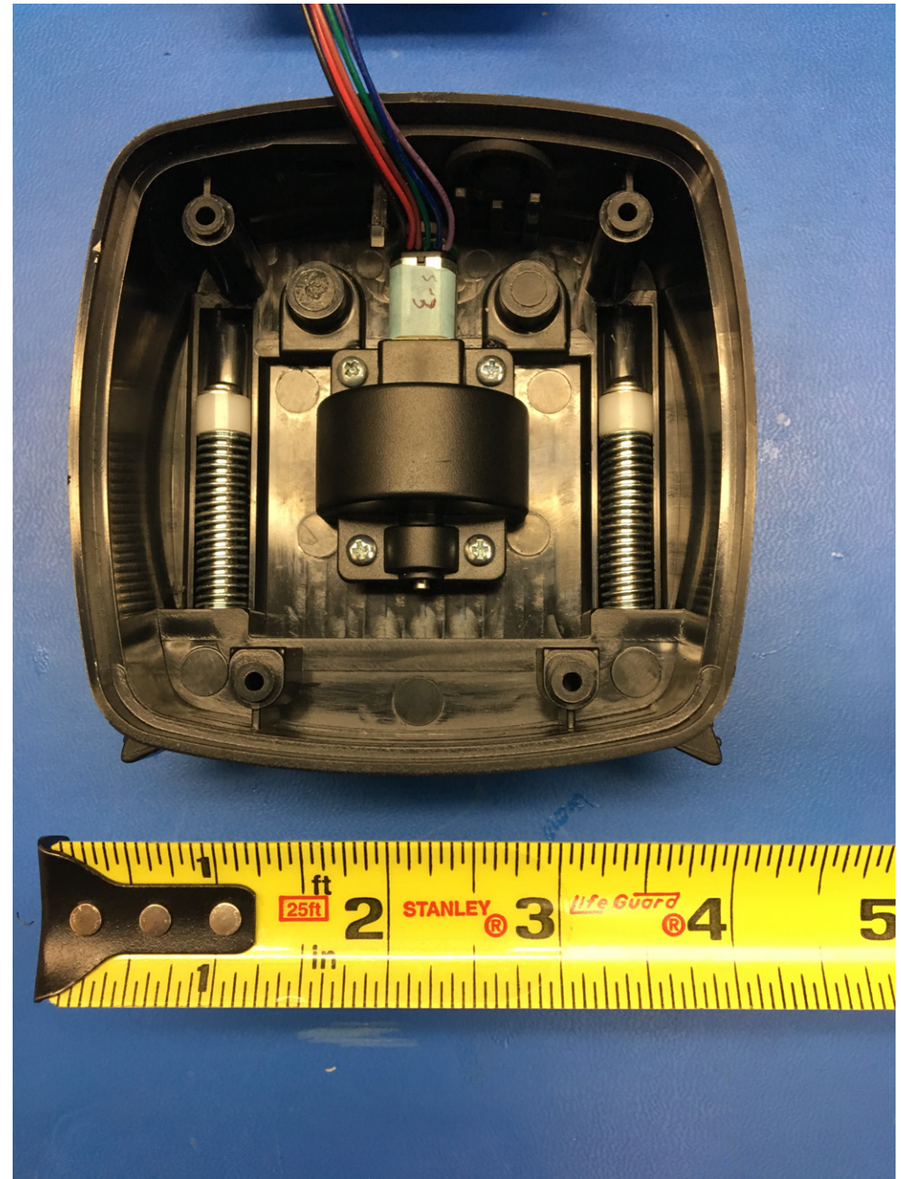
Fig 2: Top view of system with PCA removed.
