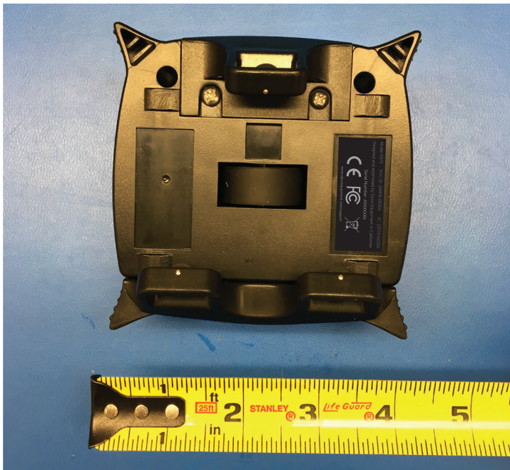
Fig 2: Bottom view of system with label drawing shown in the final label location.
