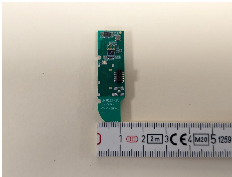
Secondary PCB Bottom View
