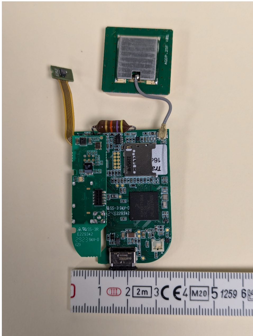
Bottom of Main and Secondary PCB
