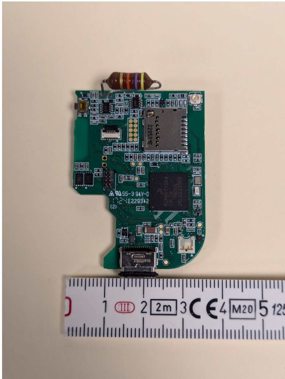
Bottom of Main PCB with Secondary PCB Removed
