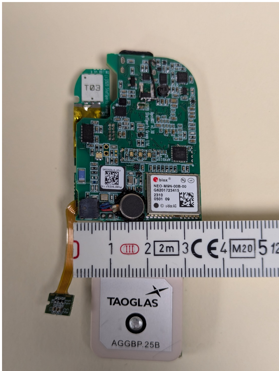
Main PCB Removed from Enclosure Top View
