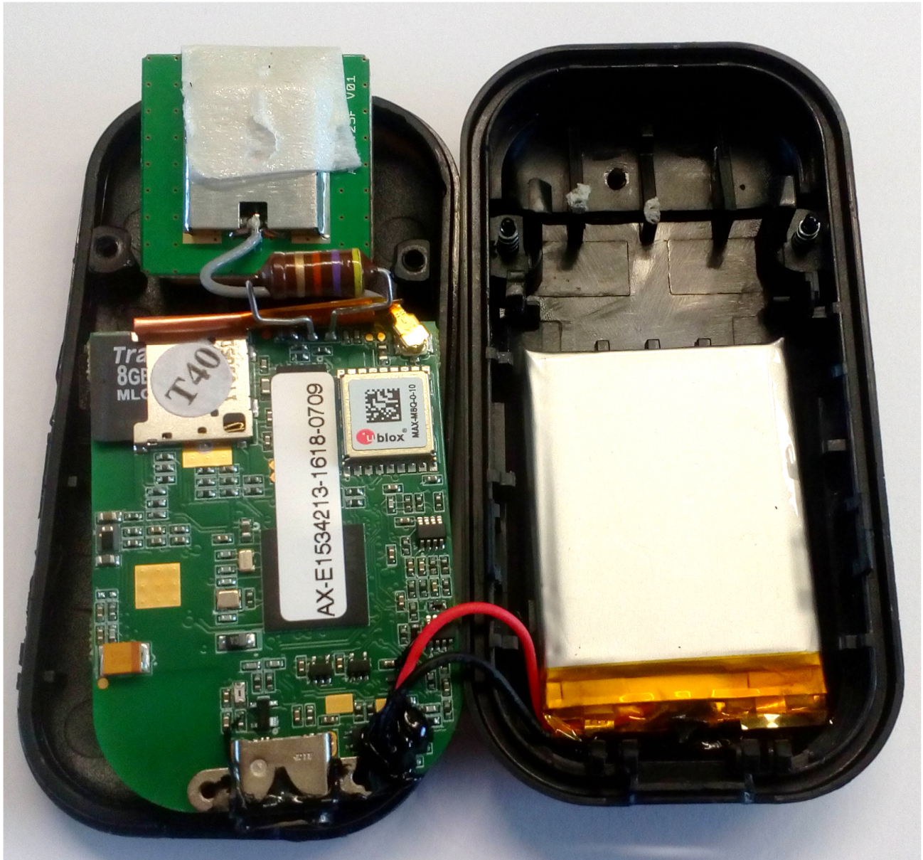
APEX PCB (REAR) Fitted in Casing
