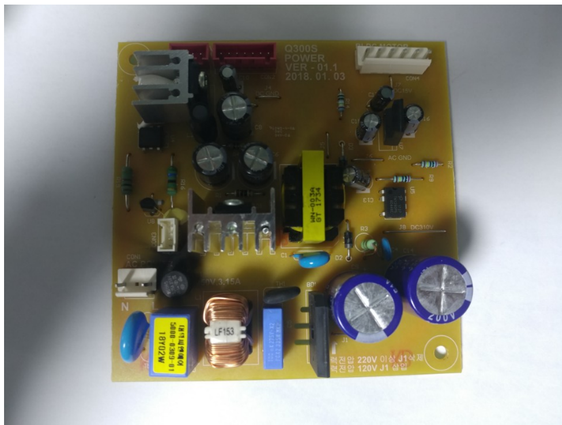
Sub Board 1 Front
