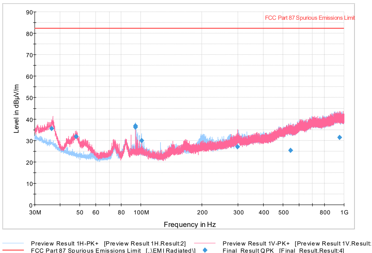
Full Spectrum
