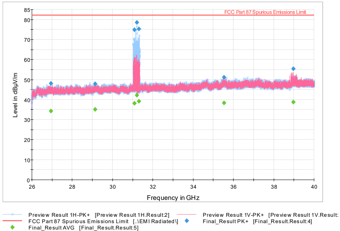
Full Spectrum
