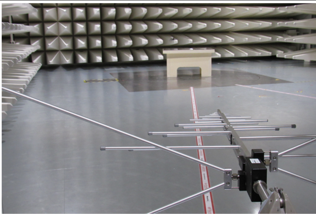
Setup Radiated Overview
