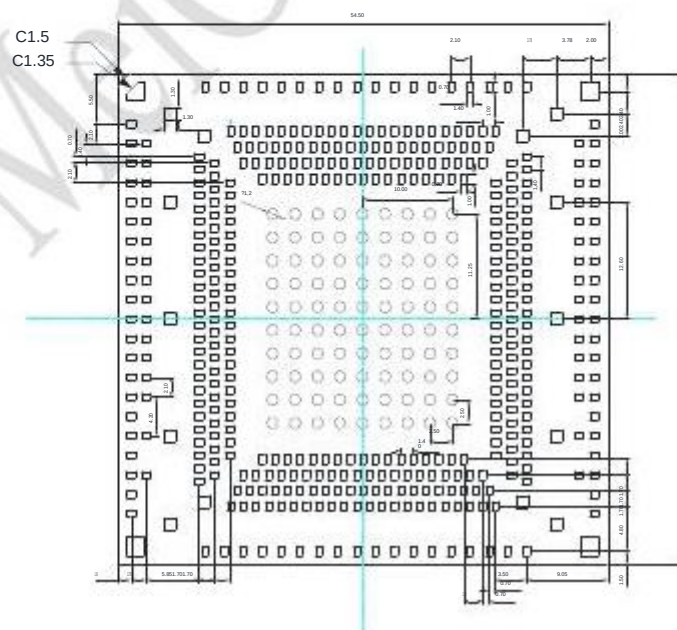
Figure 40 Bottom view dimension drawing (unit: mm)
