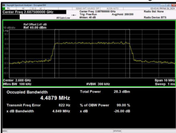
LTE Band 41 16QAM 5MHz CH-High
