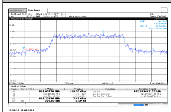
Band26-0.18-QPSK-26692-12@0-15kHz-PASS
