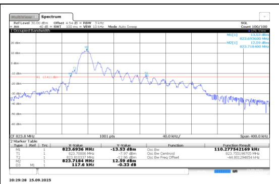
Band26-0.18-QPSK-26788-1@0-15kHz-PASS
