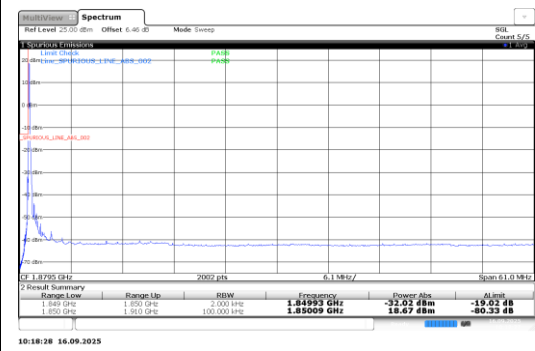
Band2-0.18-BPSK-18602-1@0-15kHz-PASS
