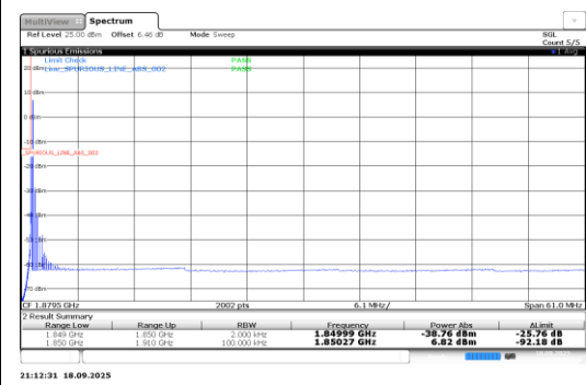
Band2-0.18-BPSK-18602-12@0-15kHz-PASS
