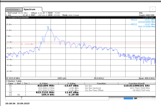
Band26-0.18-BPSK-26788-1@0-15kHz-PASS
