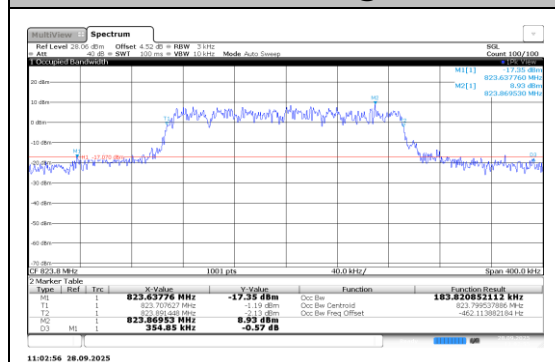
Band26-0.18-QPSK-26788-12@0-15kHz-PASS
