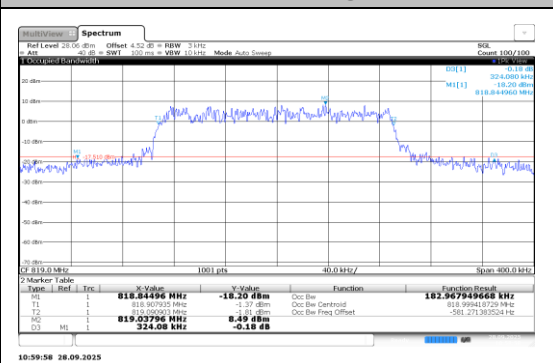
Band26-0.18-QPSK-26740-12@0-15kHz-PASS
