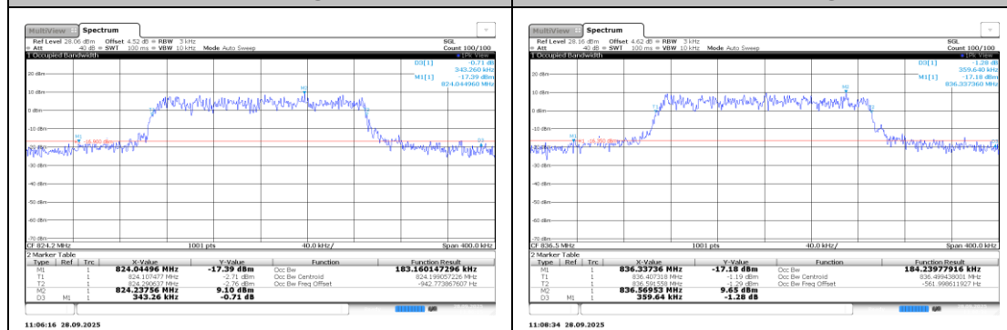
Band26-0.18-QPSK-26792-12@0-15kHz-PASS
