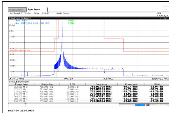
Band13-0.18-BPSK-23181-1@0-15kHz-PASS
