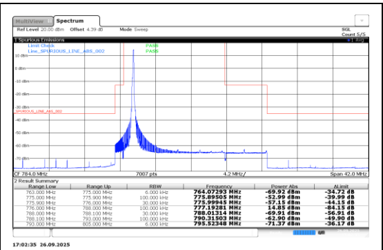
Band13-0.18-BPSK-23181-1@11-15kHz-PASS
