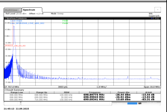
Band12-0.18-BPSK-23012-1@0-15kHz-PASS
