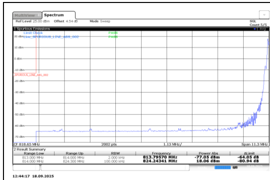
Band26-0.18-BPSK-26792-1@11-15kHz-PASS
