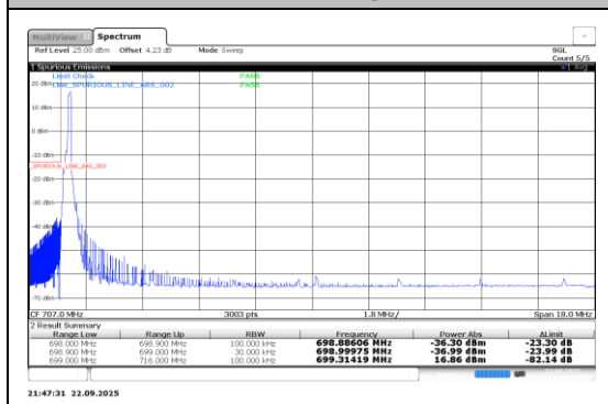
Band12-0.18-BPSK-23012-1@11-15kHz-PASS
