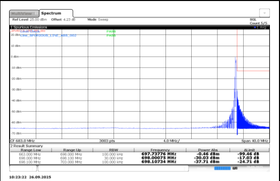
Band71-0.18-BPSK-133470-12@0-15kHz-PASS
