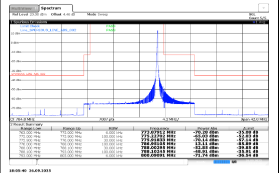
Band13-0.18-QPSK-23279-1@11-15kHz-PASS
