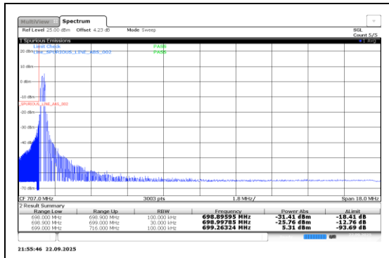
Band12-0.18-QPSK-23012-12@0-15kHz-PASS
