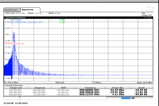
Band12-0.18-BPSK-23012-12@0-15kHz-PASS
