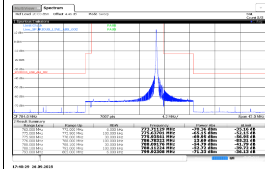
Band13-0.18-QPSK-23279-1@0-15kHz-PASS
