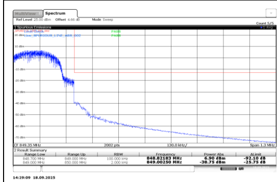
Band26-0.18-QPSK-27038-12@0-15kHz-PASS
