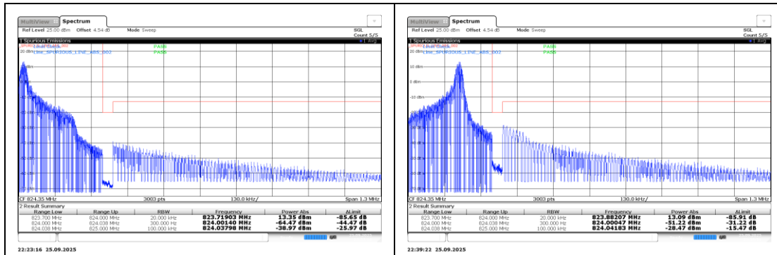
Band26-0.18-QPSK-26788-1@0-15kHz-PASS
