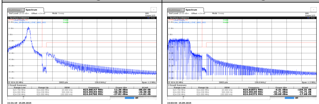
Band26-0.18-BPSK-26788-1@11-15kHz-PASS
