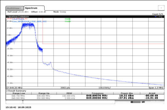
Band26-0.18-QPSK-27038-1@11-15kHz-PASS
