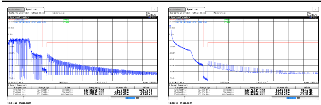
Band26-0.18-QPSK-26788-12@0-15kHz-PASS
