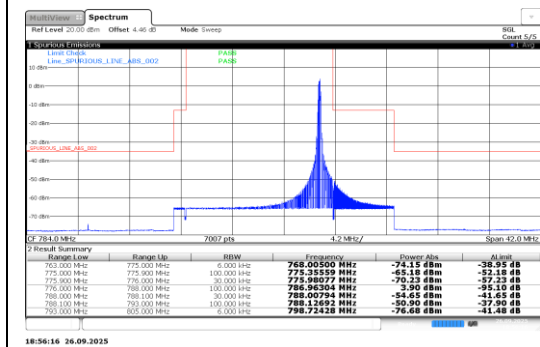
Band13-0.18-QPSK-23279-12@0-15kHz-PASS
