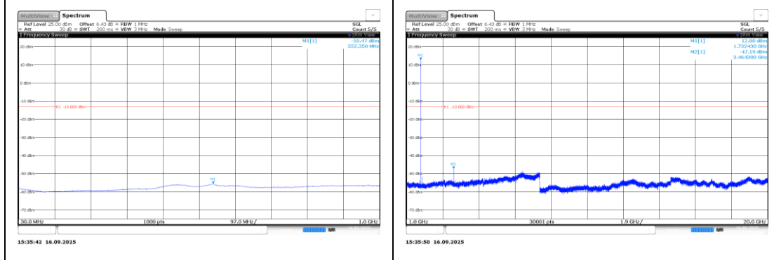
Band4-0.18-BPSK-20175-1@0-15kHz-30-1000-PASS Band4-0.18-BPSK-20175-1@0-15kHz-1000-20000-PASS
