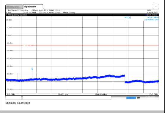
Band5-0.18-BPSK-20648-1@11-15kHz-1000-10000-PASS
