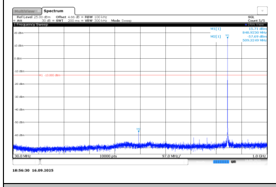
Band5-0.18-BPSK-20648-1@11-15kHz-30-1000-PASS
