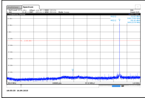
Band5-0.18-BPSK-20648-1@0-15kHz-30-1000-PASS
