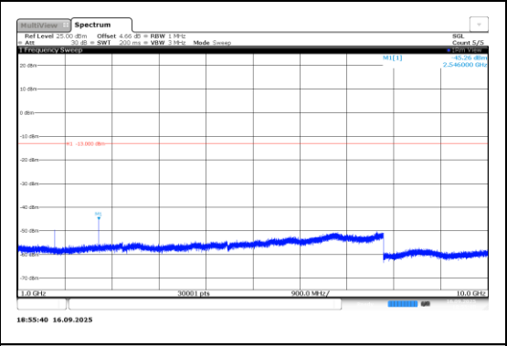
Band5-0.18-BPSK-20648-1@0-15kHz-1000-10000-PASS
