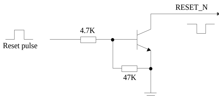
Figure 9. RESET_N reset the open set reference circuit
